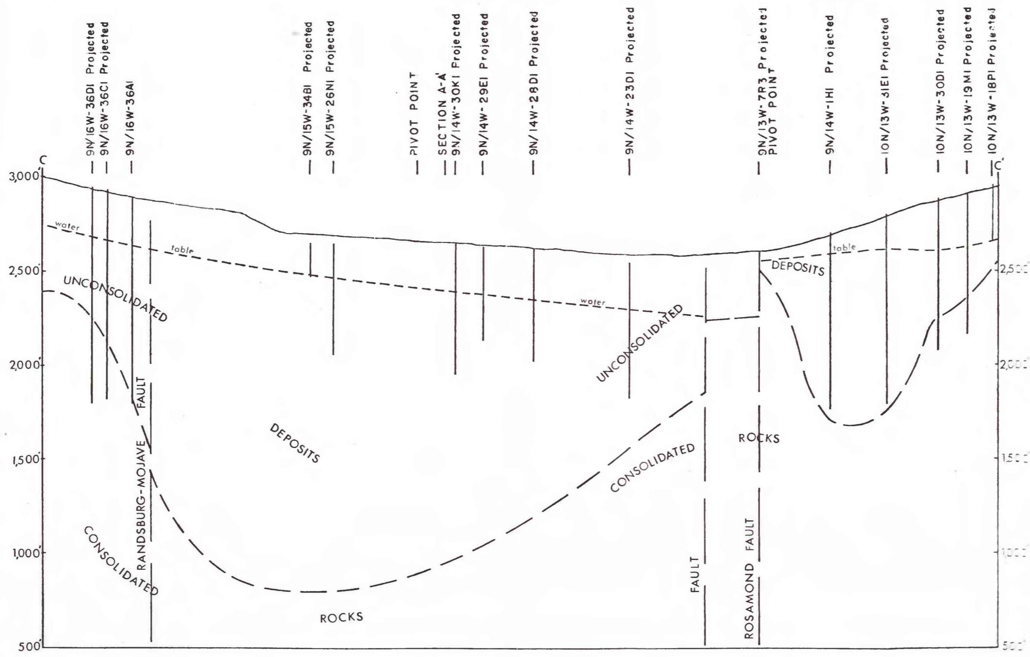
GEOLOGIC SECTION C-C' IN ANTELOPE VALLEY SHOWING WATER-LEVEL PROFILE
