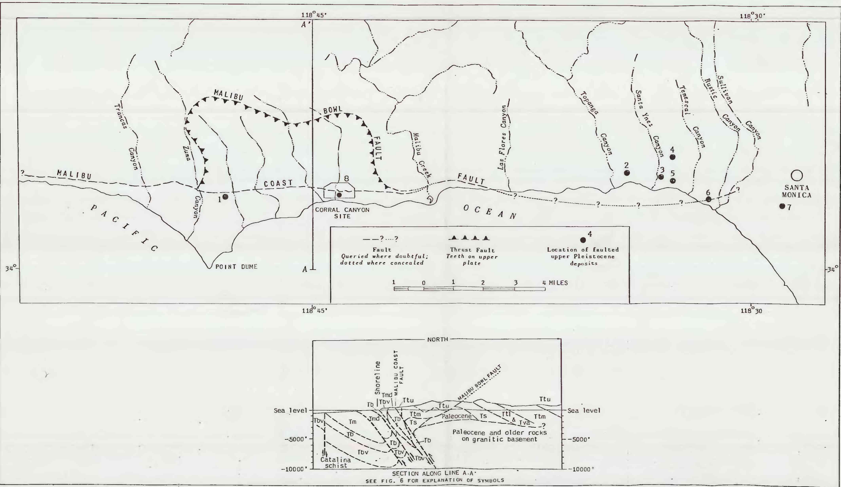
Fig. 3. Outline map of central Santa Monica Mountains showing Malibu Coast and Malibu Bowl faults, and locations of faulted upper Pleistocene deposits
