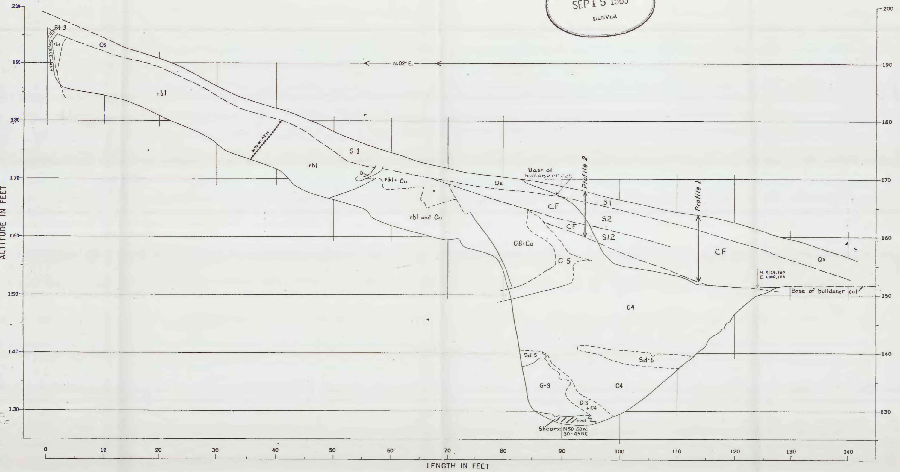
FIG. 13 TEST TRENCH E-MAP OF VERTICAL EAST FACE
