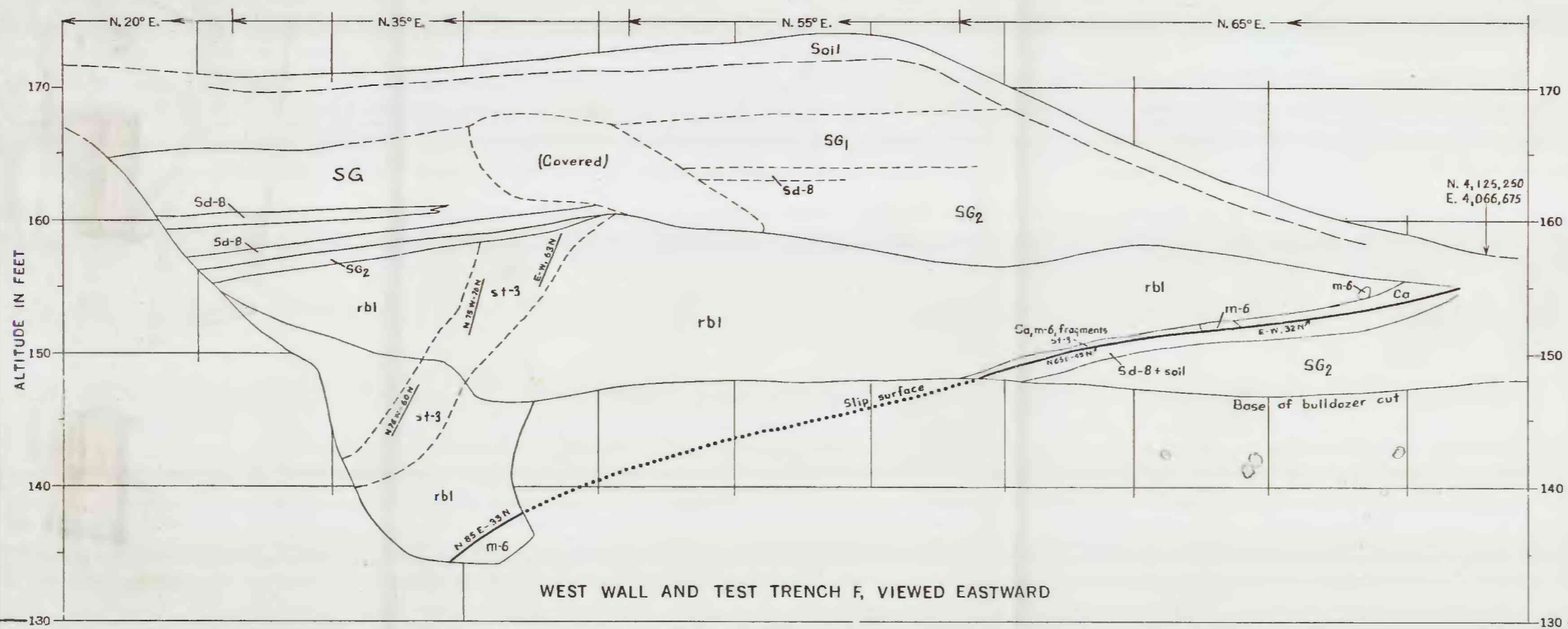
FIG.14 TEST TRENCH F AND GULLY C-MAPS OF WALLS
