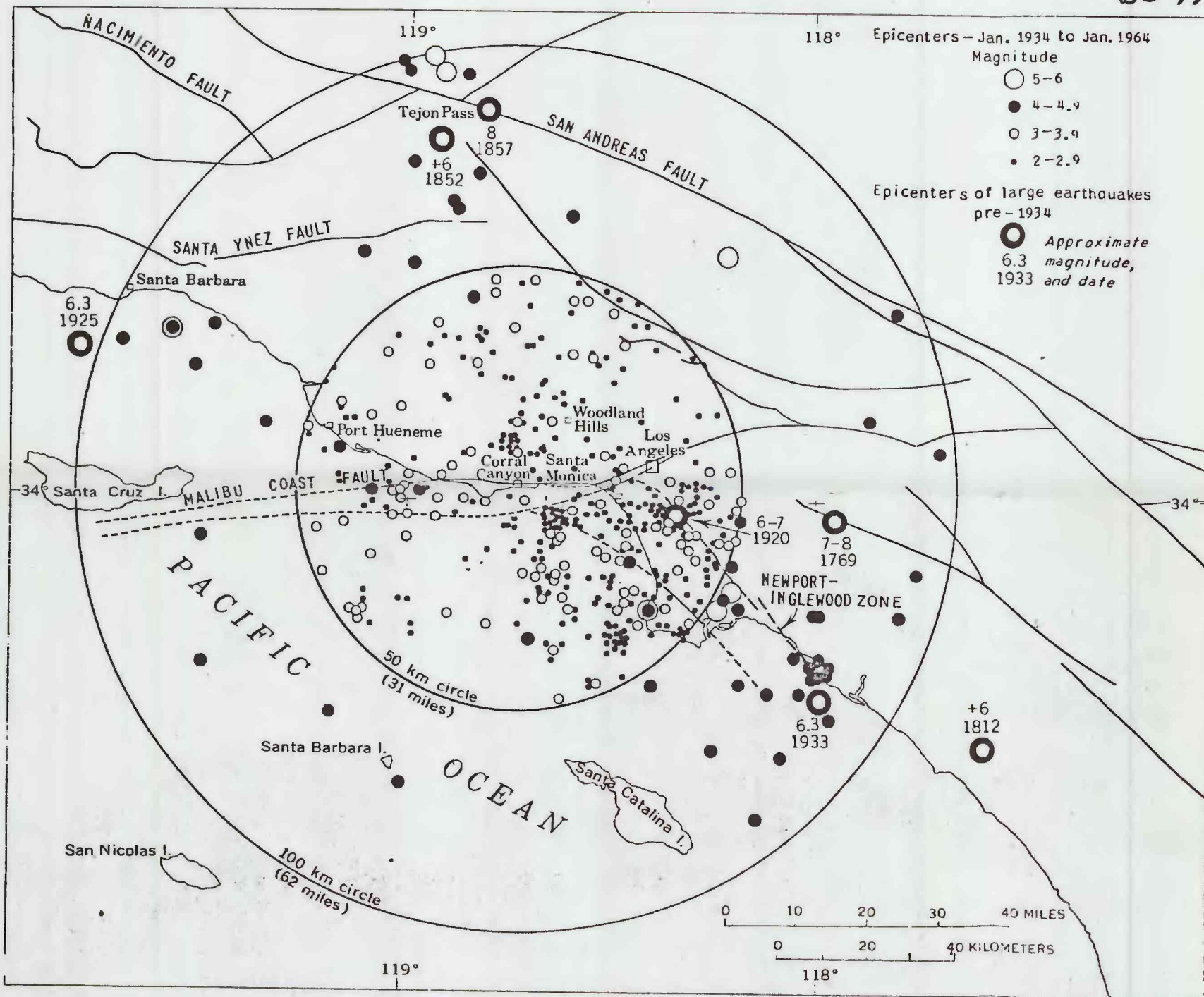
Fig. 44. Known post-1933 seismic epicenters, magnitude 2 and greater, within 50 km. of the Corral Canyon site and all known epicenters, magnitude 4 and greater, within 100 km. of the site, showing relation to larger faults of southern California. Post-1933 epicenters compiled by J. H. Healy of the U.S. Geological Survey from records of California Institute of Technology. Most epicenters are located within 5 to 15 km; within the 50-km. circle those of magnitude 4 and greater on land or along fault zones are located within 5 km. Pre-1934 epicenters from Richter(1958).
