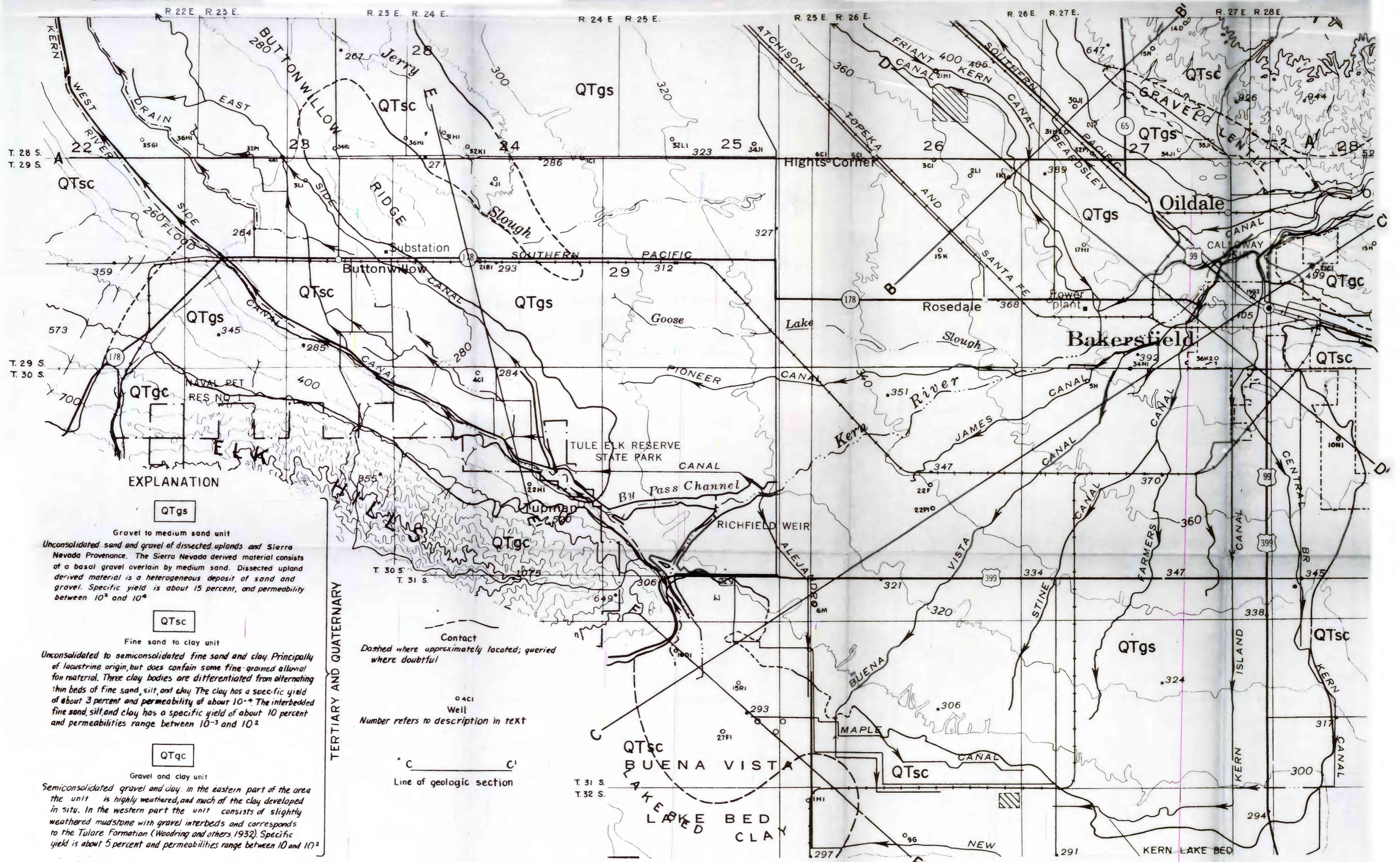
FIGURE 7a—GEOLOGIC MAP OF ROCK-STRATIGRAPHIC UNITS
