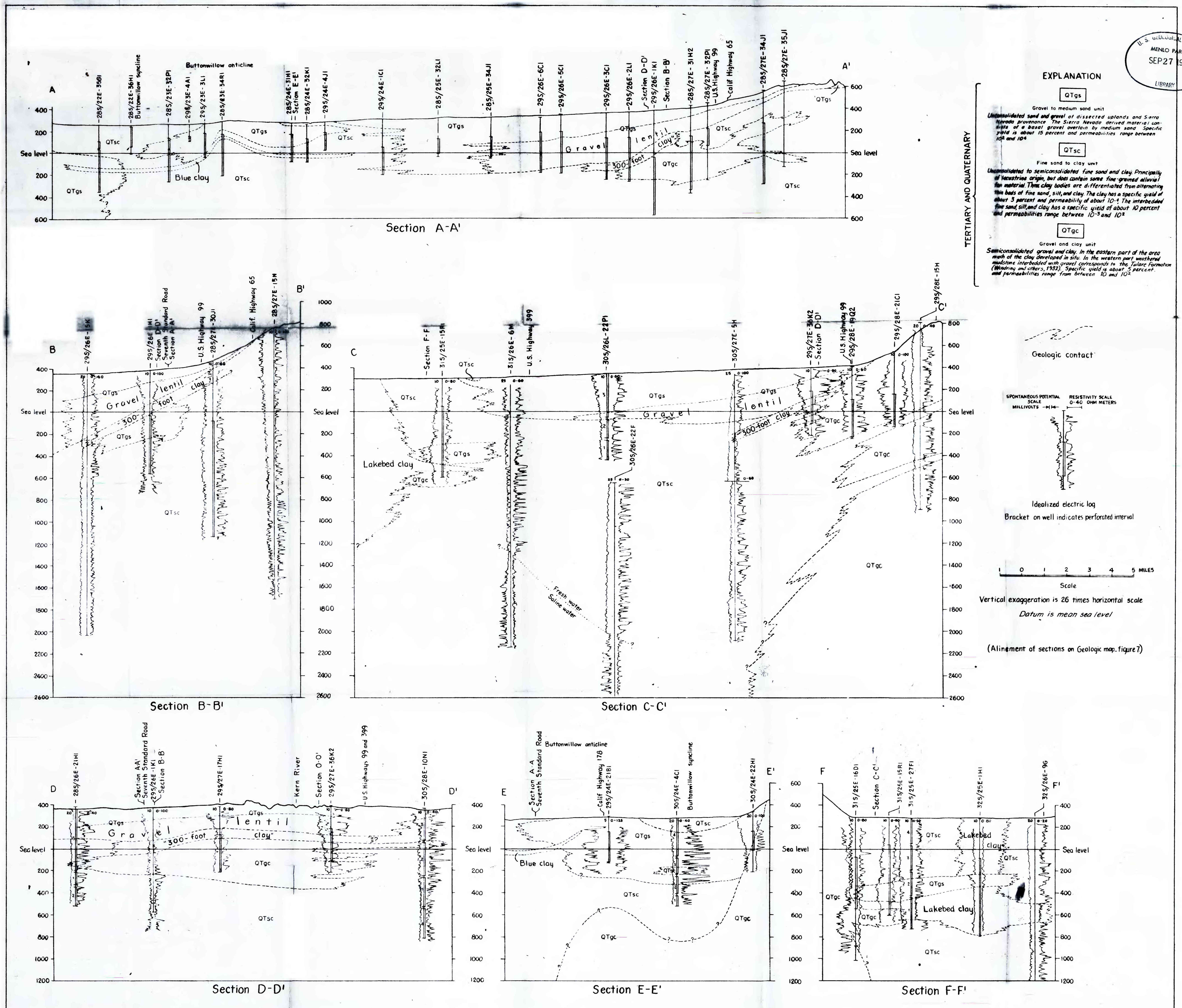
FIGURE 10.—GEOLOGIC SECTIONS A-A', B-B', C-C', D-D', E-E', F-F' KERN RIVER ALLUVIAL-FAN AREA, CALIFORNIA
