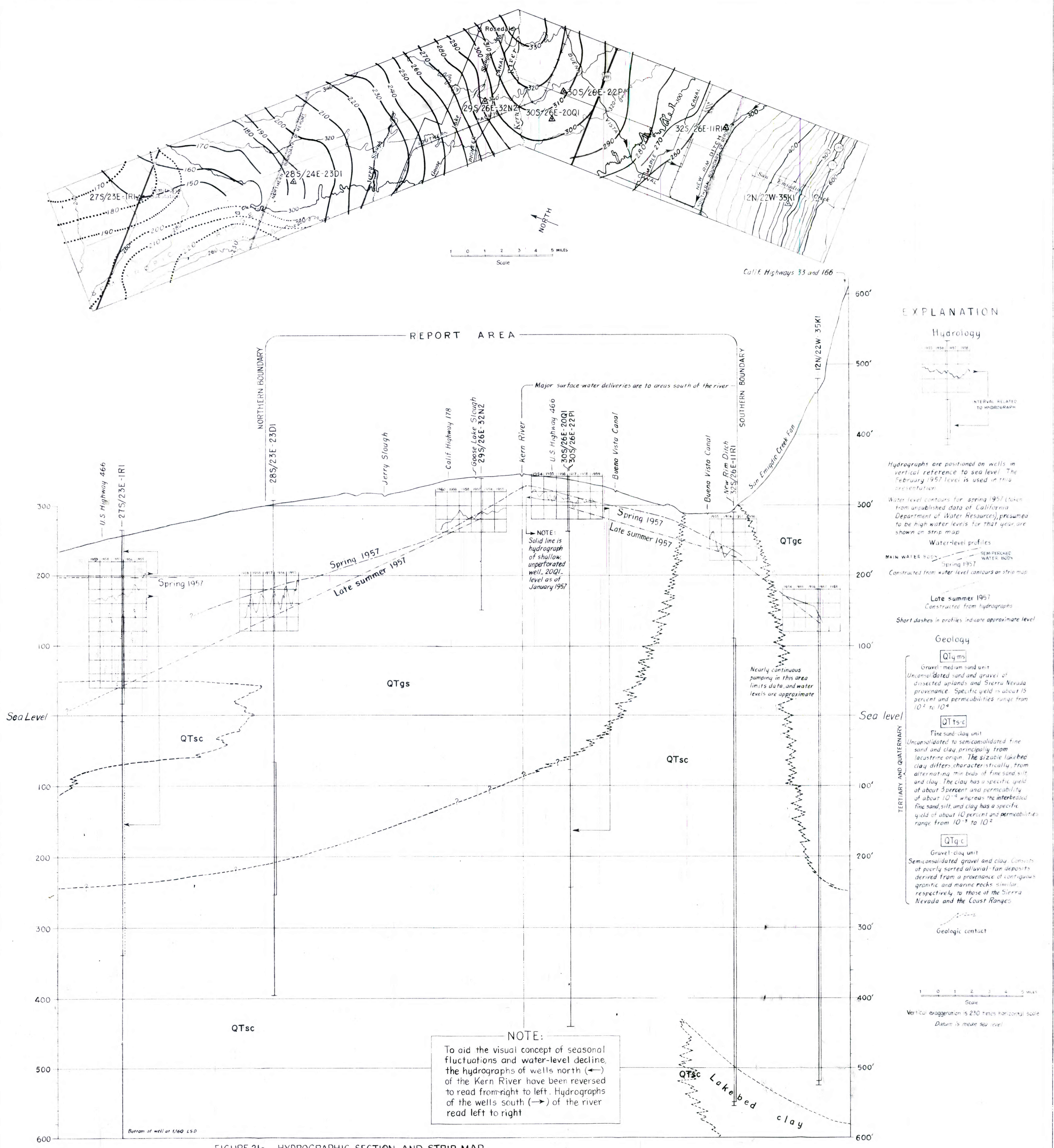
FIGURE 21a. HYDROGRAPHIC SECTION AND STRIP MAP PART OF KERN RIVER ALLUVIAL-FAN AREA AND ADJACENT AREAS, CALIFORNIA
