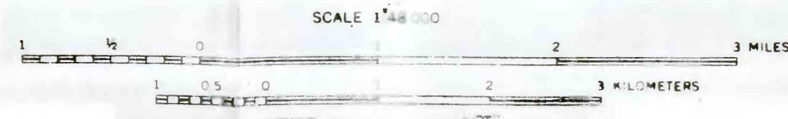
MAP SHOWING GEOLOGY AND LOCATION OF SELECTED WELLS, LOMPOC SUBAREA, SANTA YNEZ RIVER BASIN, CALIFORNIA, 1957-62
