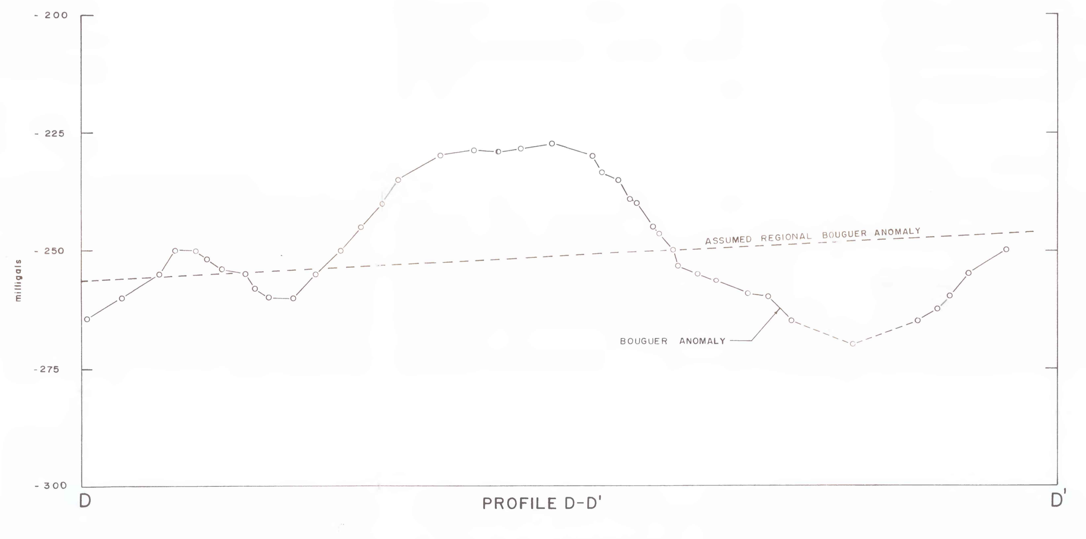
Figure 4 GRAVITY PROFILES COMPLETE BOUGUER VALUES SAN LUIS VALLEY, COLORADO
