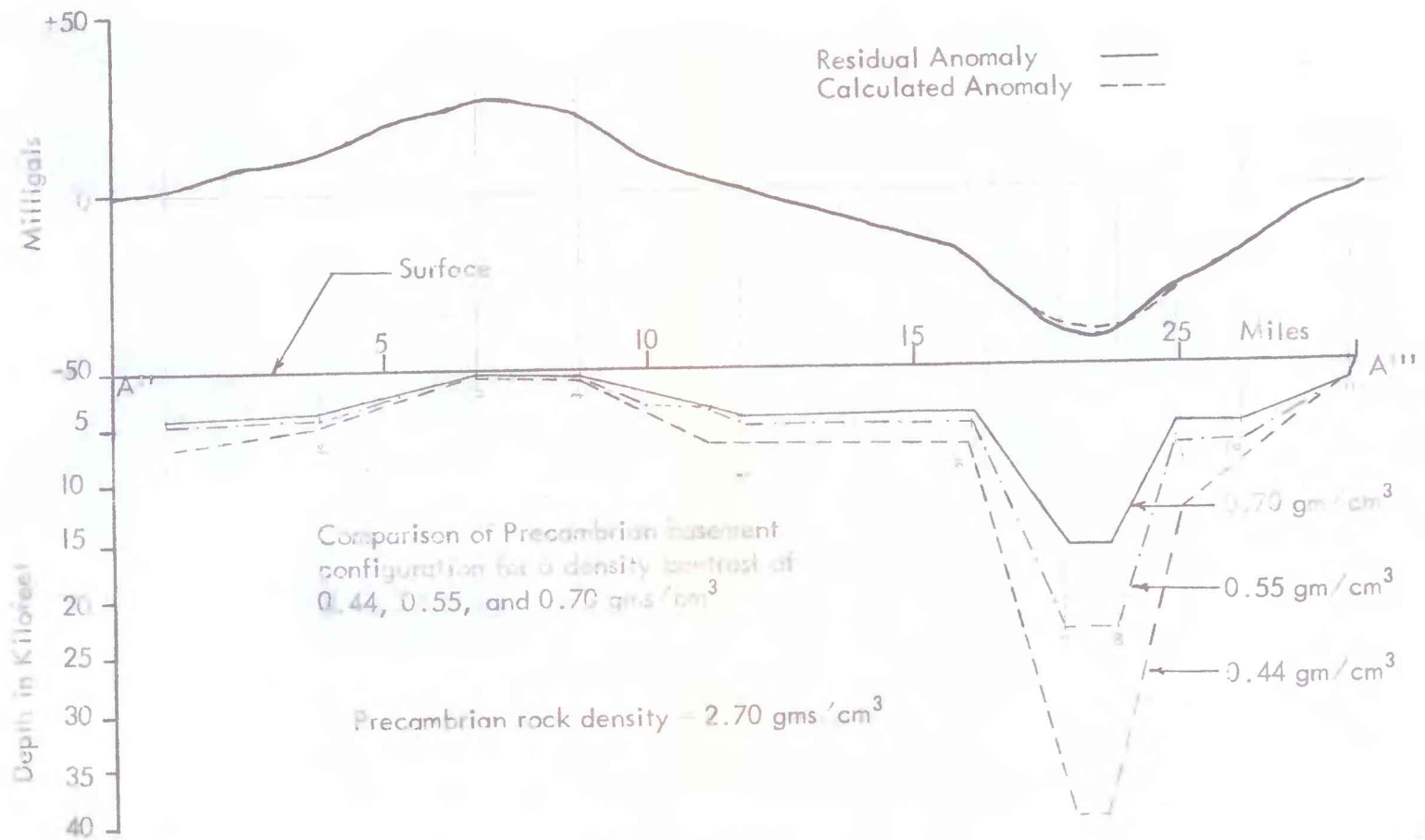
Figure 5- Interpretive Profile A'' - A'''
