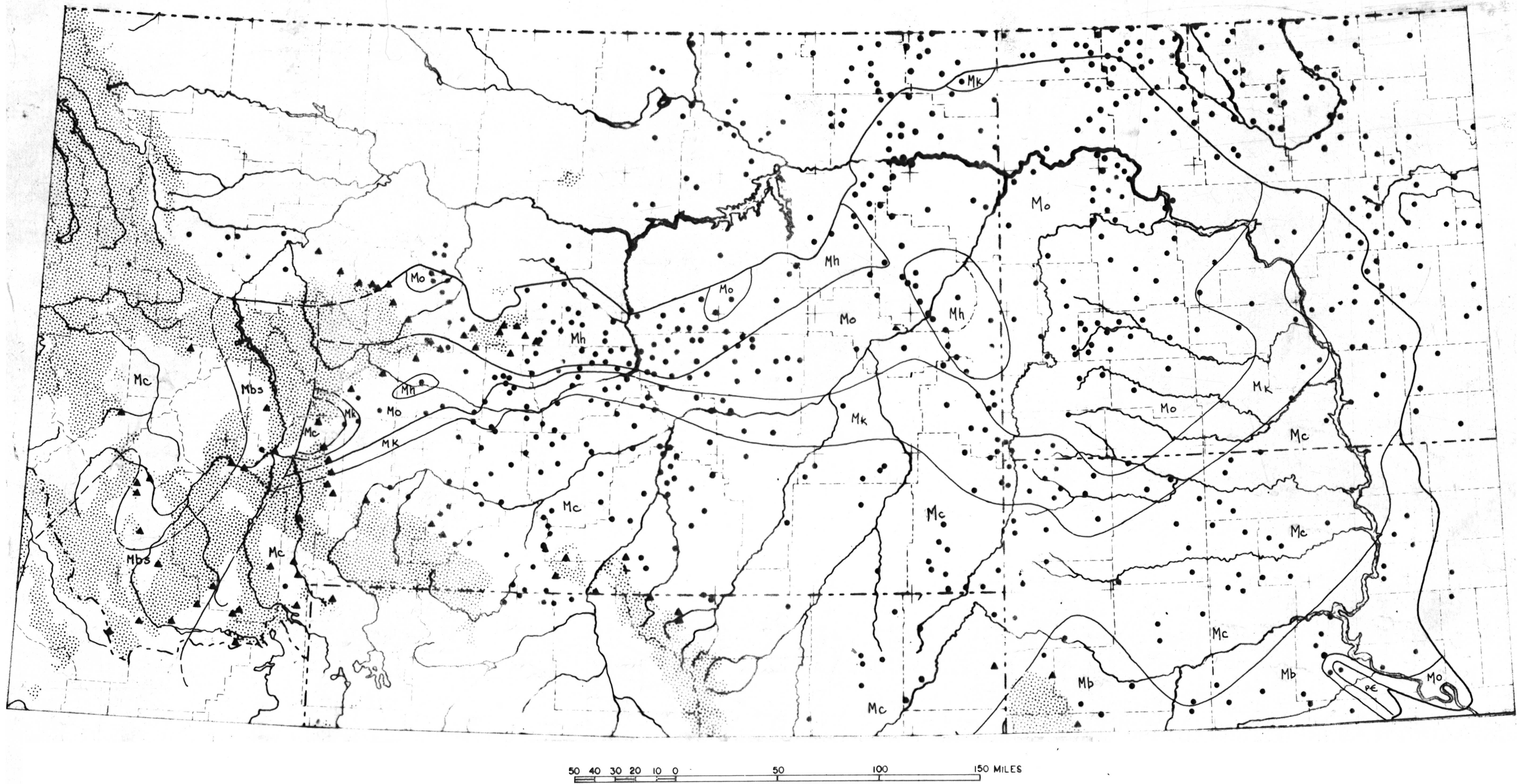
Figure 1. Preliminary map showing paleogeology beneath Pennsylvanian rocks in Montana and parts of adjacent states
