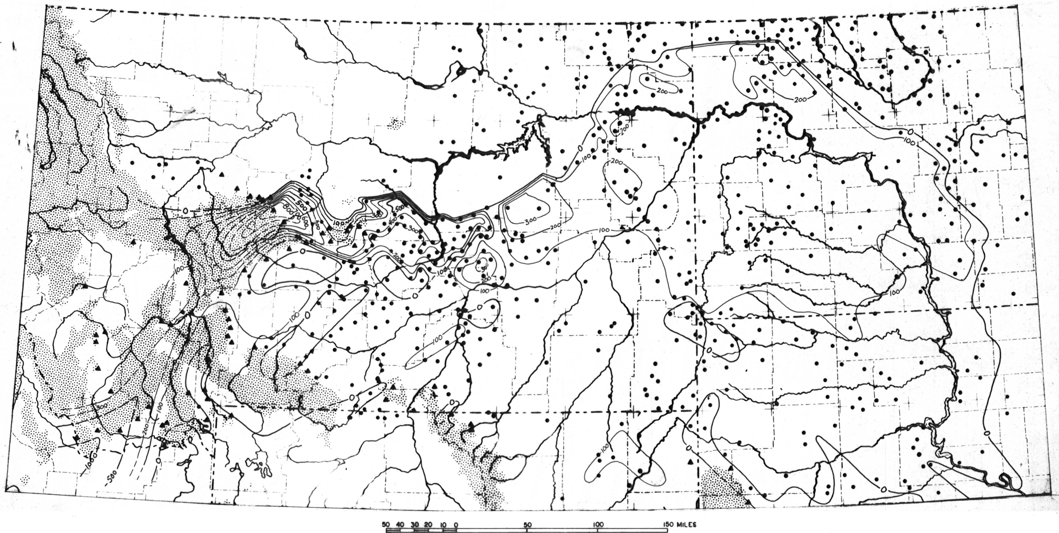
Figure 2. Preliminary map showing thickness of Pennsylvanian interval A in Montana and parts of adjacent states
