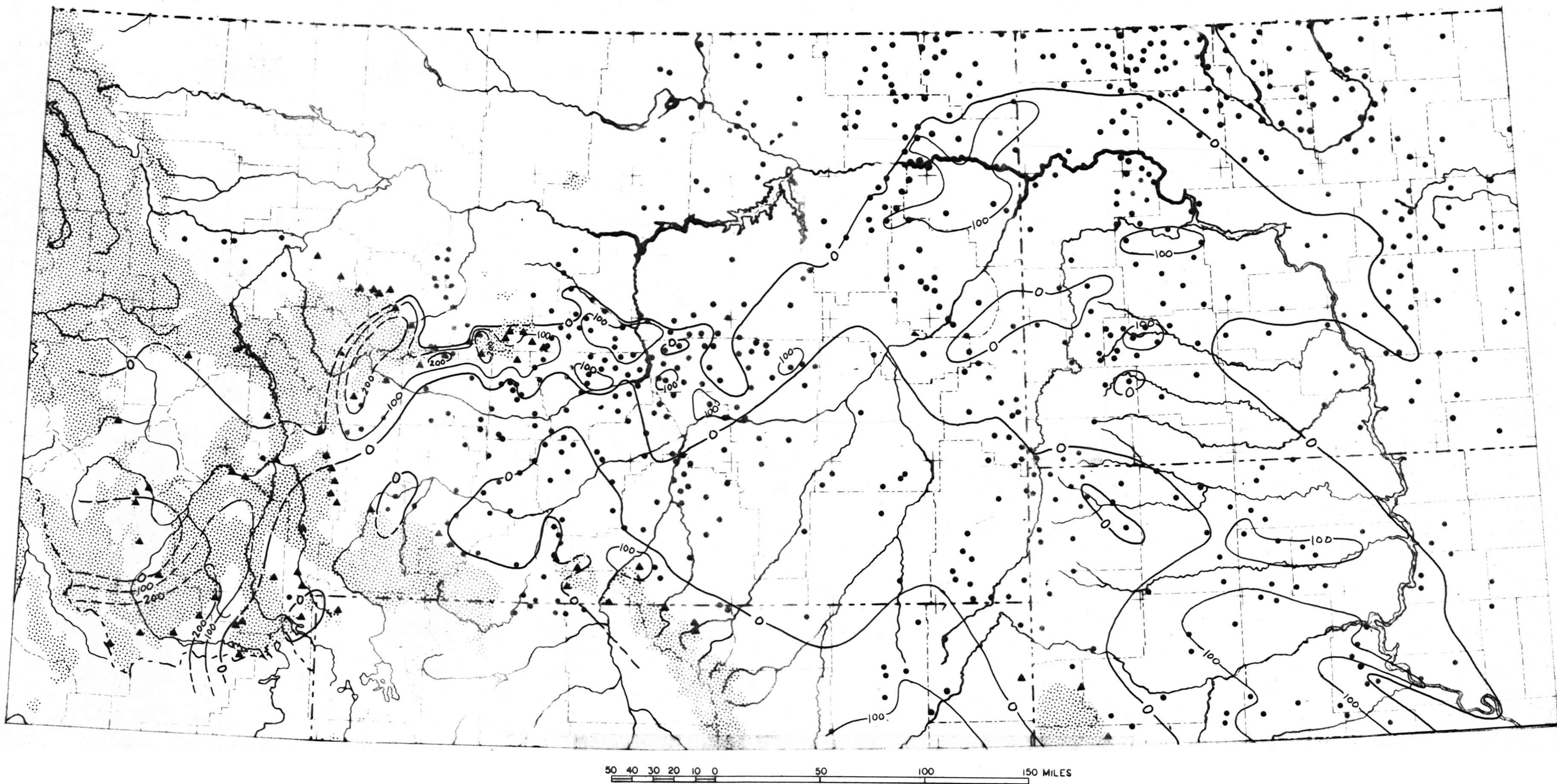
Figure 4. Preliminary map showing thickness of Pennsylvanian interval B in Montana and parts of adjacent states
