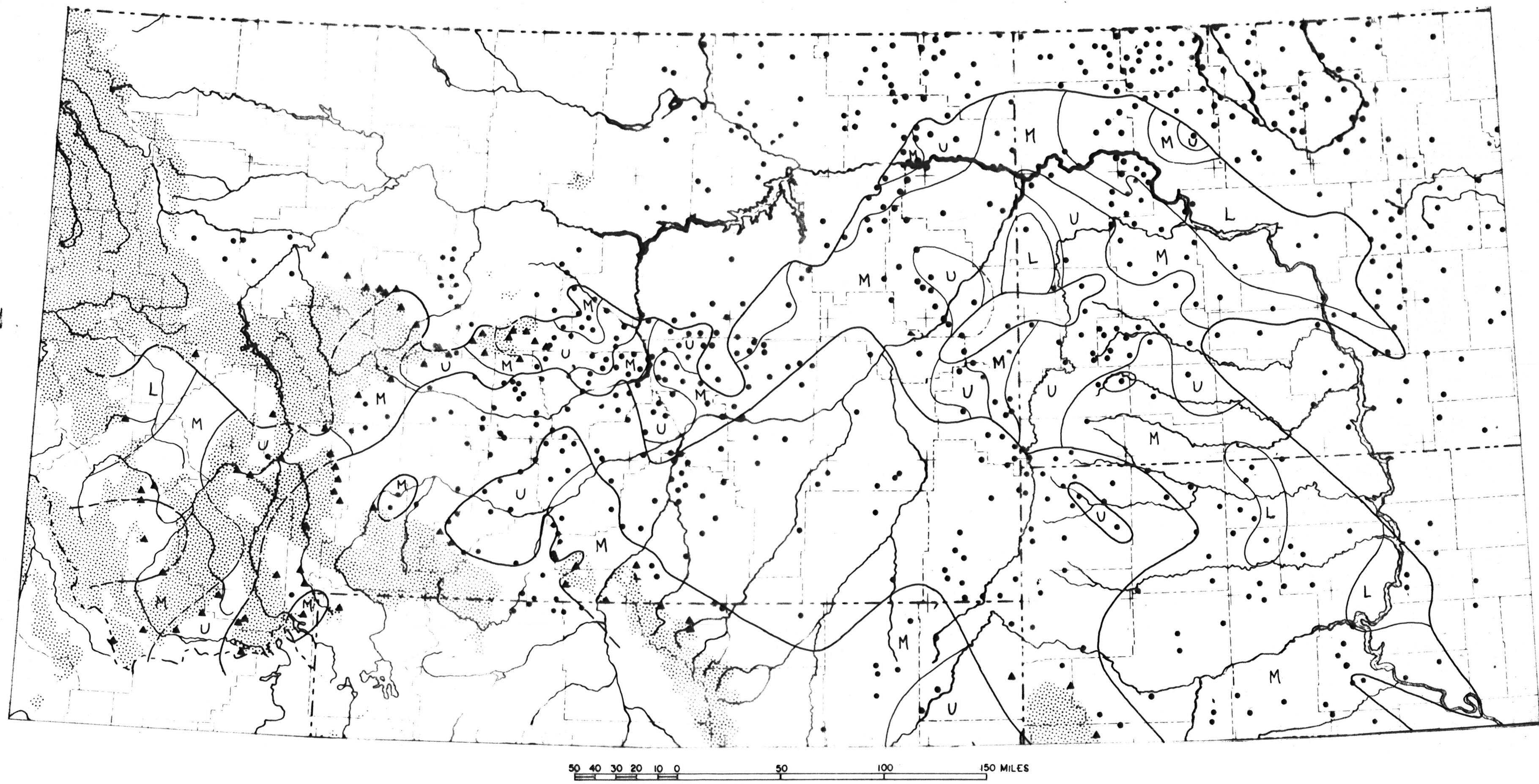
Figure 5. Preliminary map showing lithofacies of Pennsylvanian interval B in Montana and parts of adjacent states
