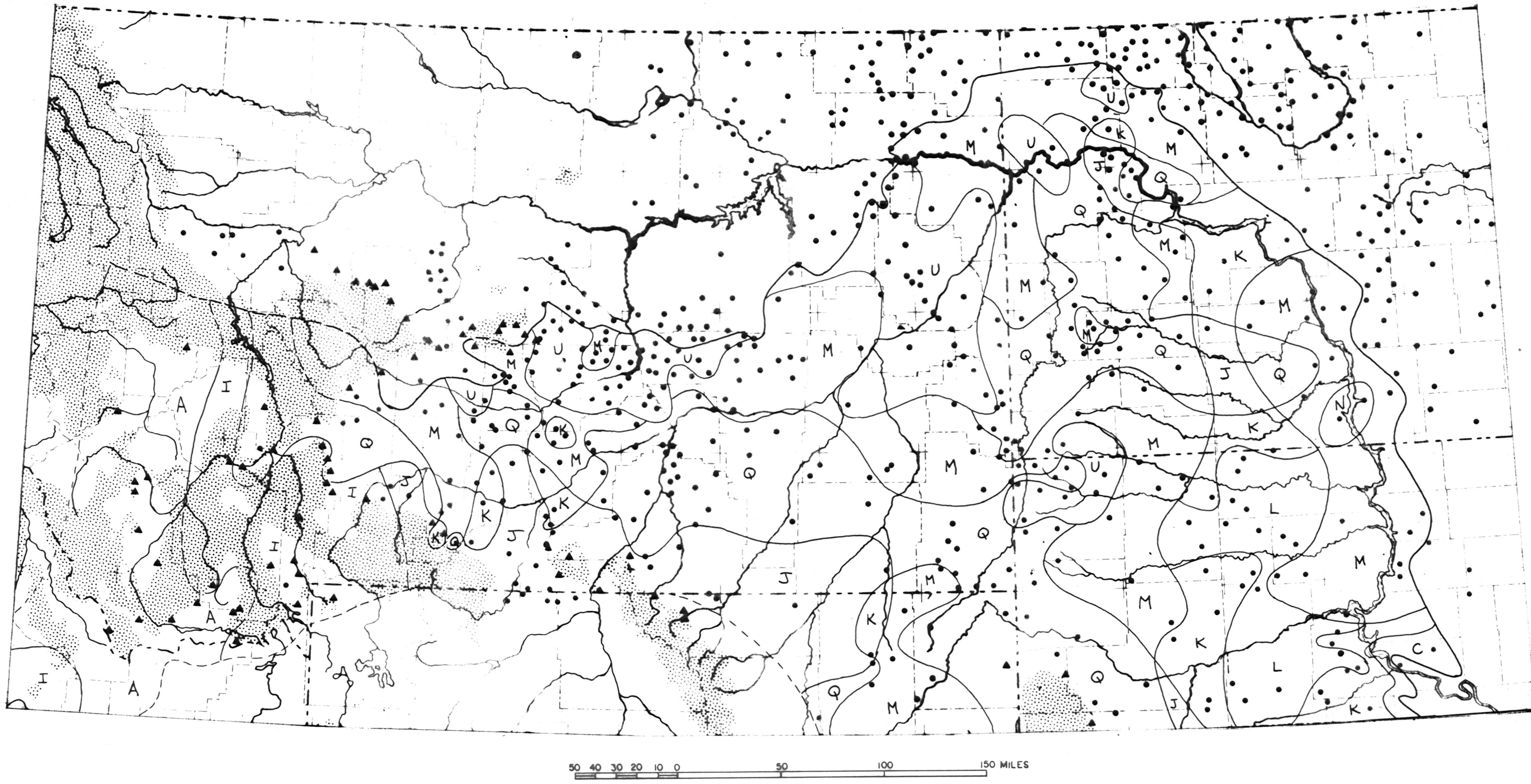
Figure 7. Preliminary map showing lithofacies of Pennsylvanian interval C in Montana and parts of adjacent states
