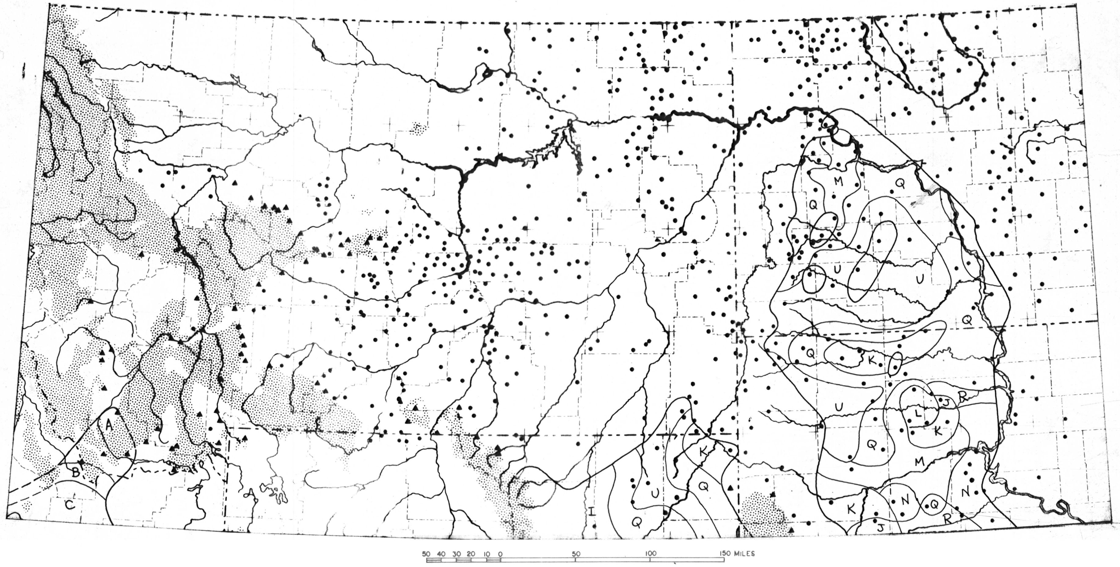
Figure 9. Preliminary map showing lithofacies of Pennsylvanian interval D in Montana and parts of adjacent states By E.K. Maughan
