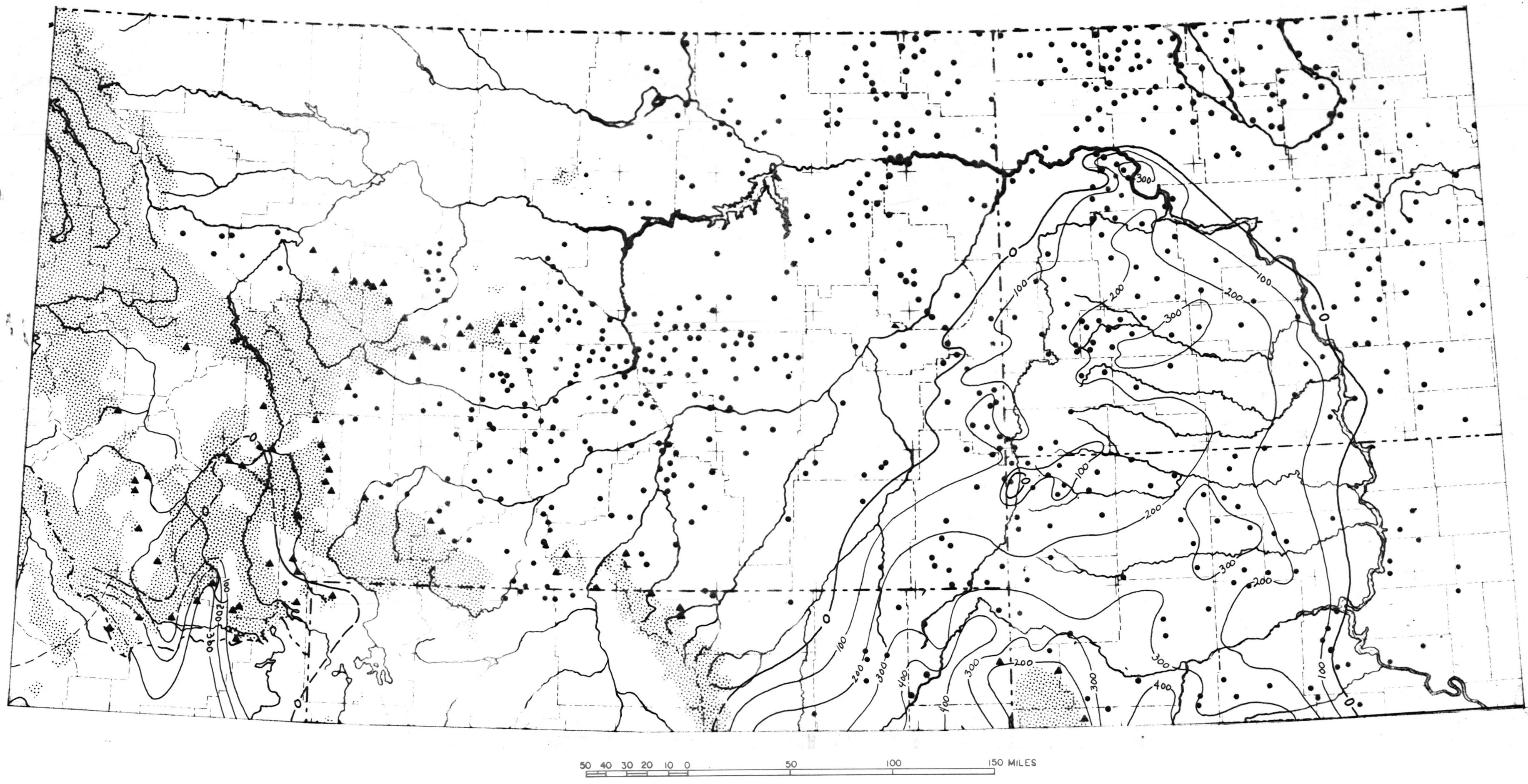
Figure 10. Preliminary map showing thickness of Permian interval A in Montana and parts of adjacent states
