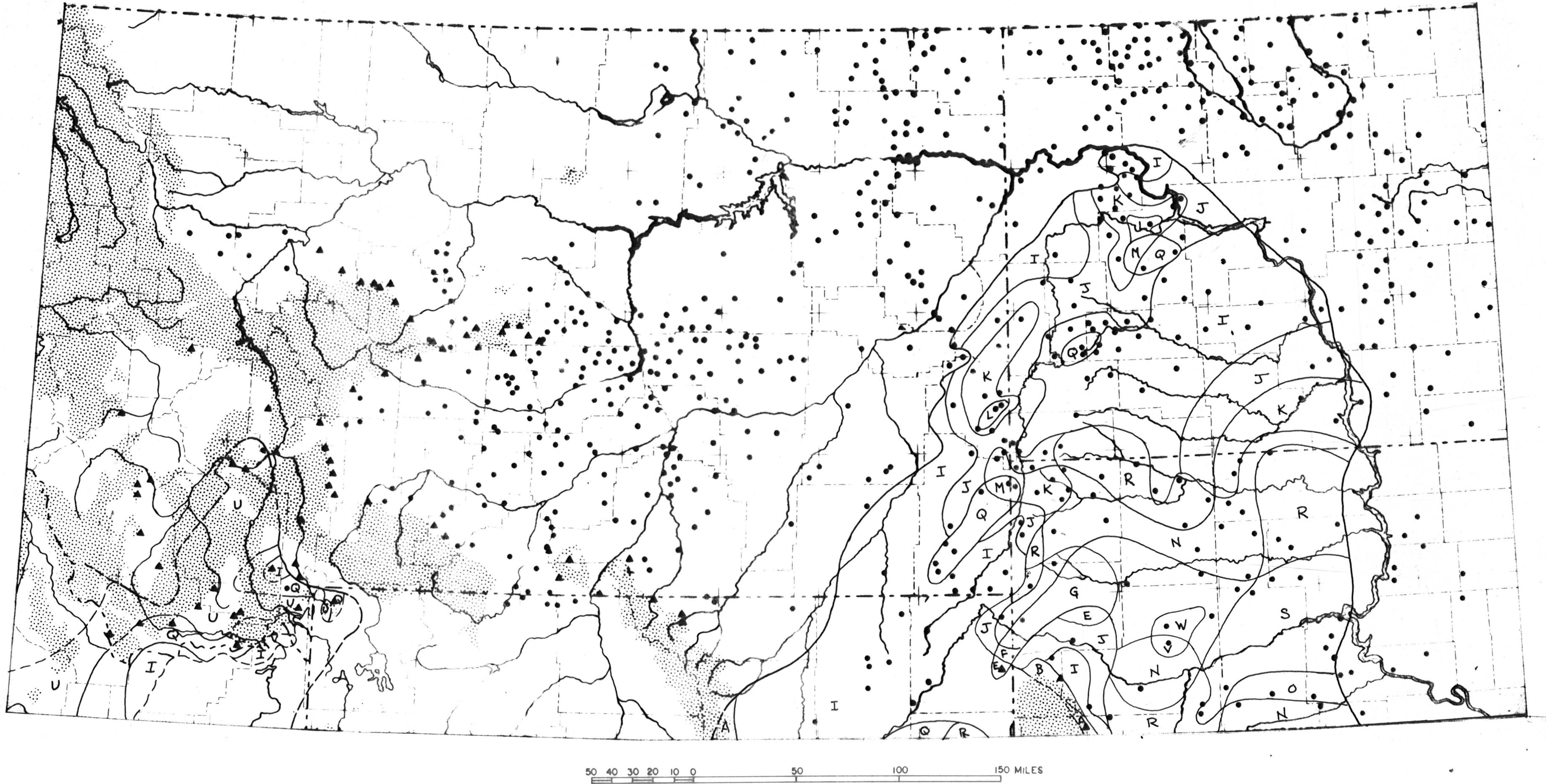
Figure 11. Preliminary map showing lithofacies of Permian interval A in Montana and parts of adjacent states
