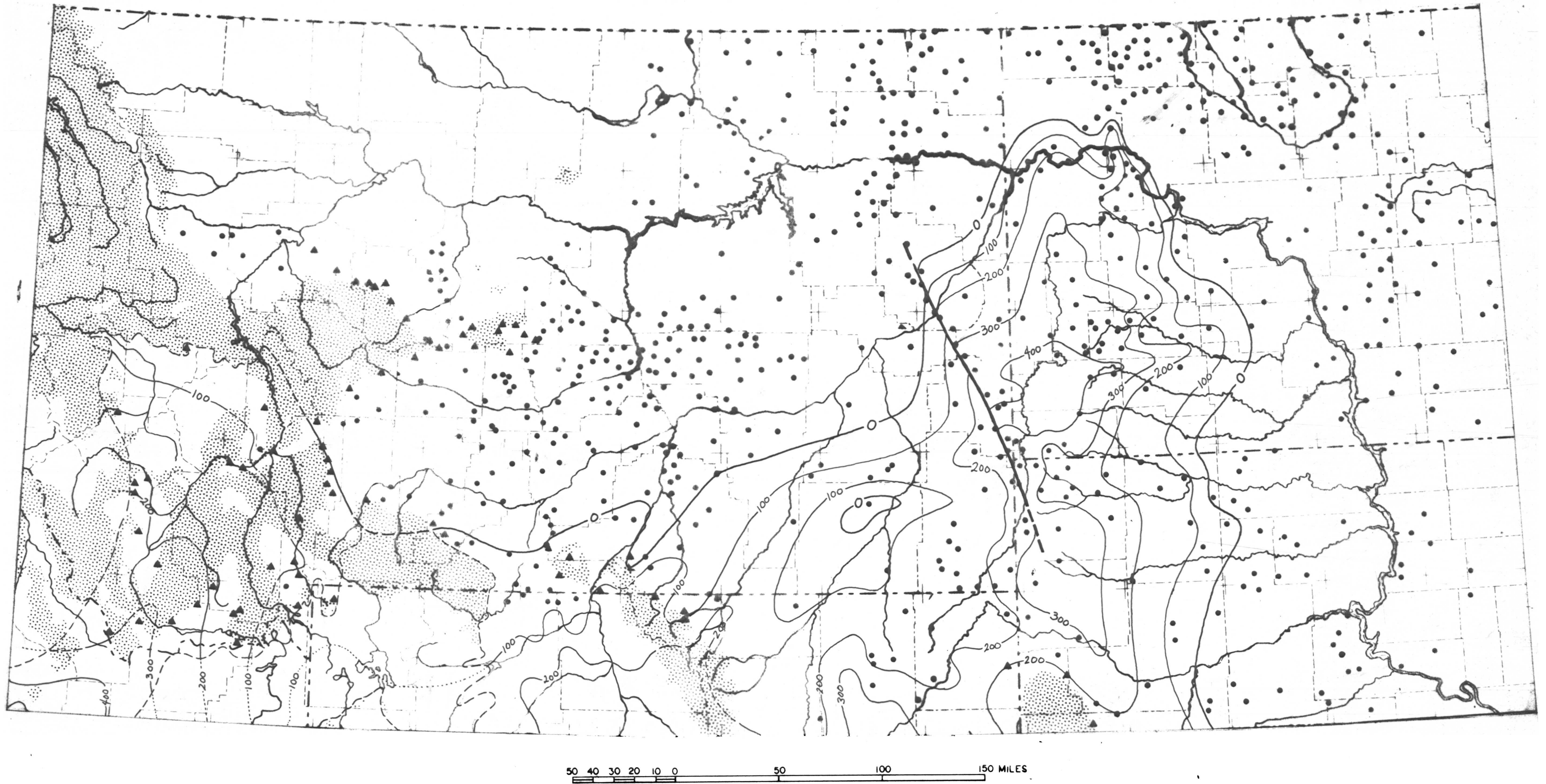
Figure 14. Preliminary map showing thickness of Permian interval C-D in Montana and parts of adjacent states
