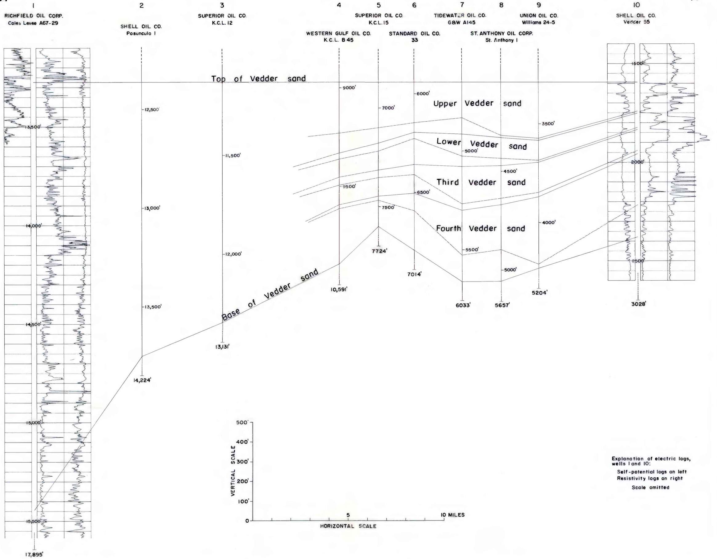
FIGURE 3.—Section along part of line A-A' (see plate i) showing correlation of members of Vedder sand.
