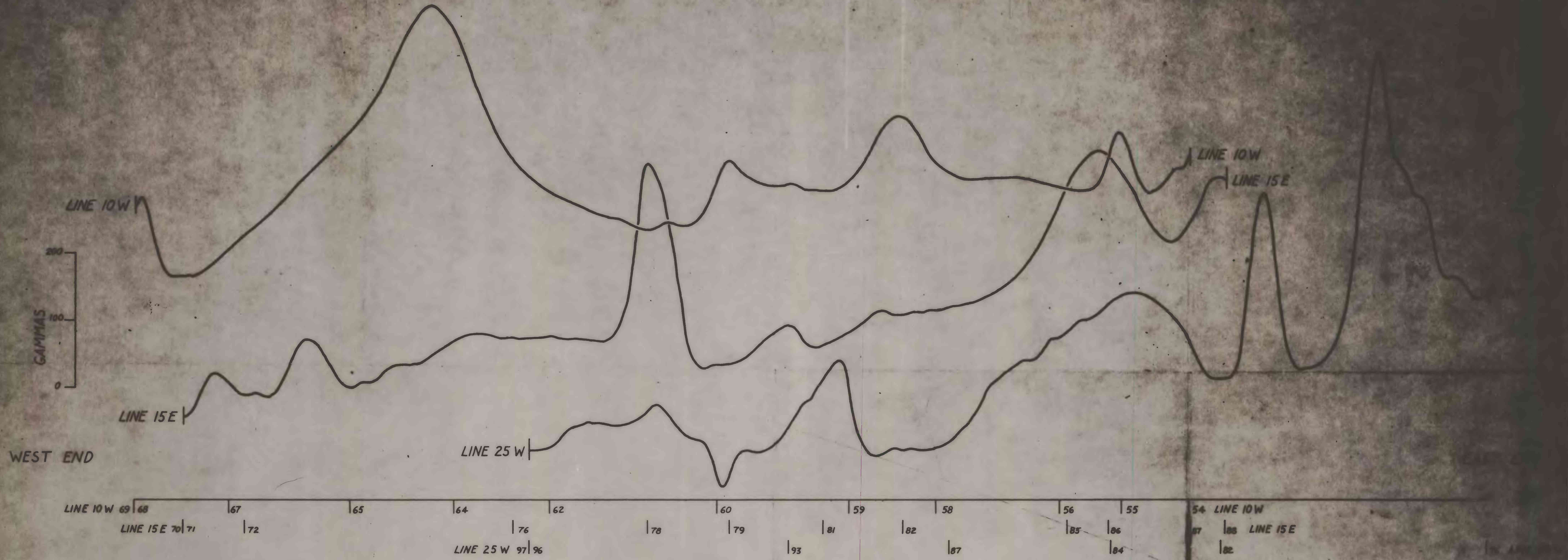
Three aeromagnetic profiles in the Bitterroot Valley area, Montana and Idaho 5 0 5 10 15 20 MILES SCALE 1:250,000 PROJECT FLOWN AT 10,500 FEET BAROMETRIC ELEVATION. U. S. GEOLOGICAL SURVEY
