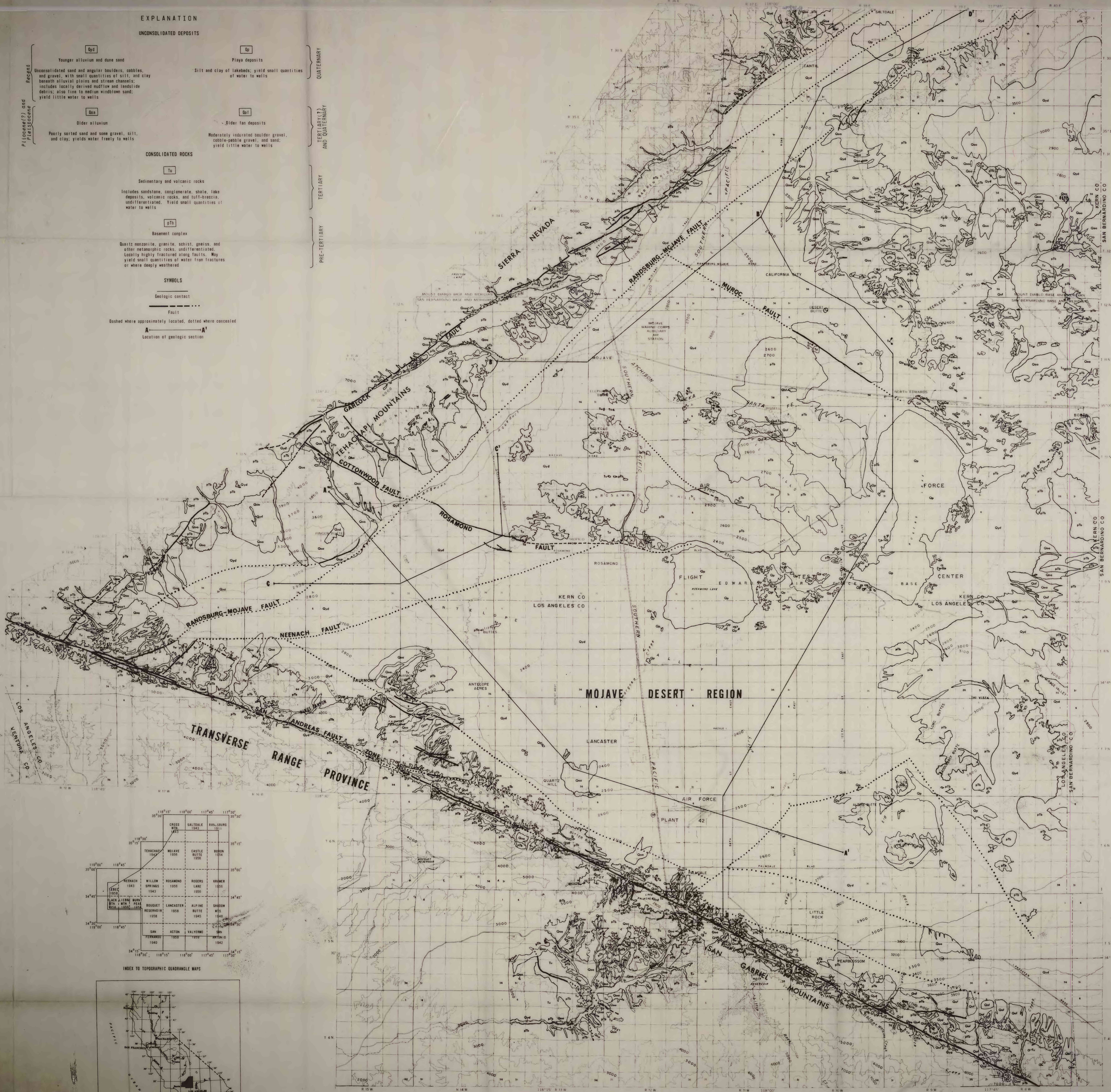
MAP OF THE ANTELOPE VALLEY-EAST KERN WATER AGENCY AREA, CALIFORNIA SHOWING GENERALIZED GEOLOGY
