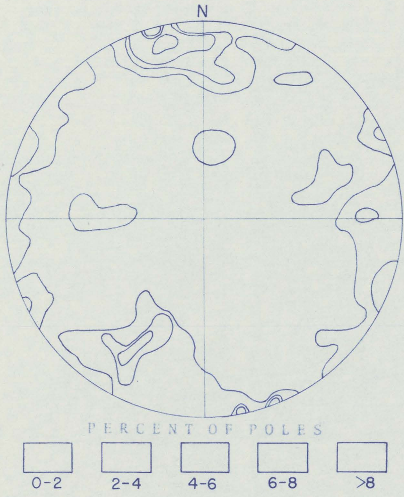
Figure 6 - Contour diagram of poles of 127 joints measured in the Tye Lake powersite area. Poles plotted on lower hemisphere. Contoured on percent of poles. (Billings, 1954, p. 108-114)
