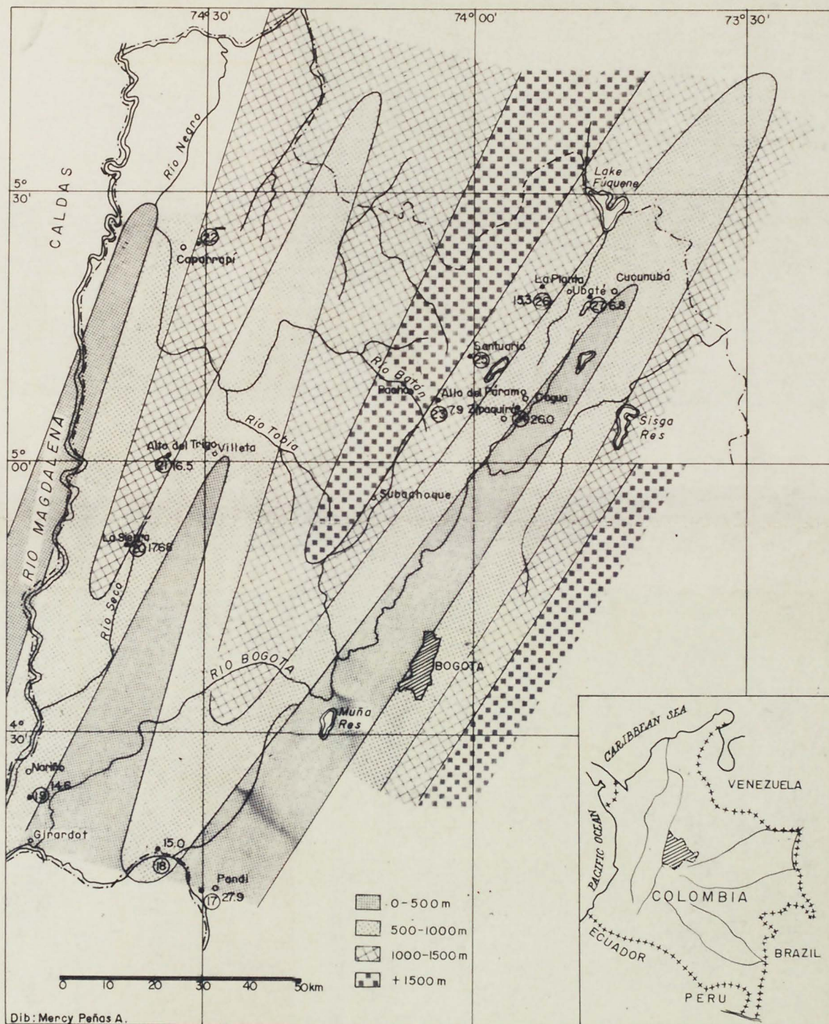
Figure 3. Isopach map of the Senonian, Department of Cundinamarca, showing relation to phosphate occurrences.
