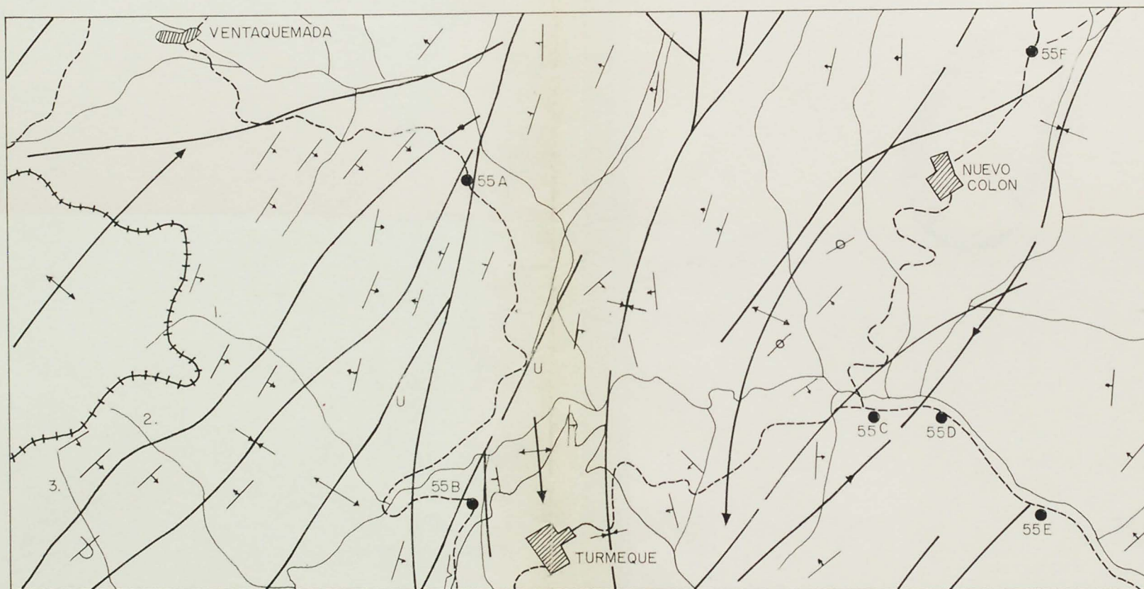
FIGURE II Photogeologic map of the TURMEQUE area, showing phosphate samples (Modified from map by Geophoto, Inc. Sample location by PEDRO MOJICA )
