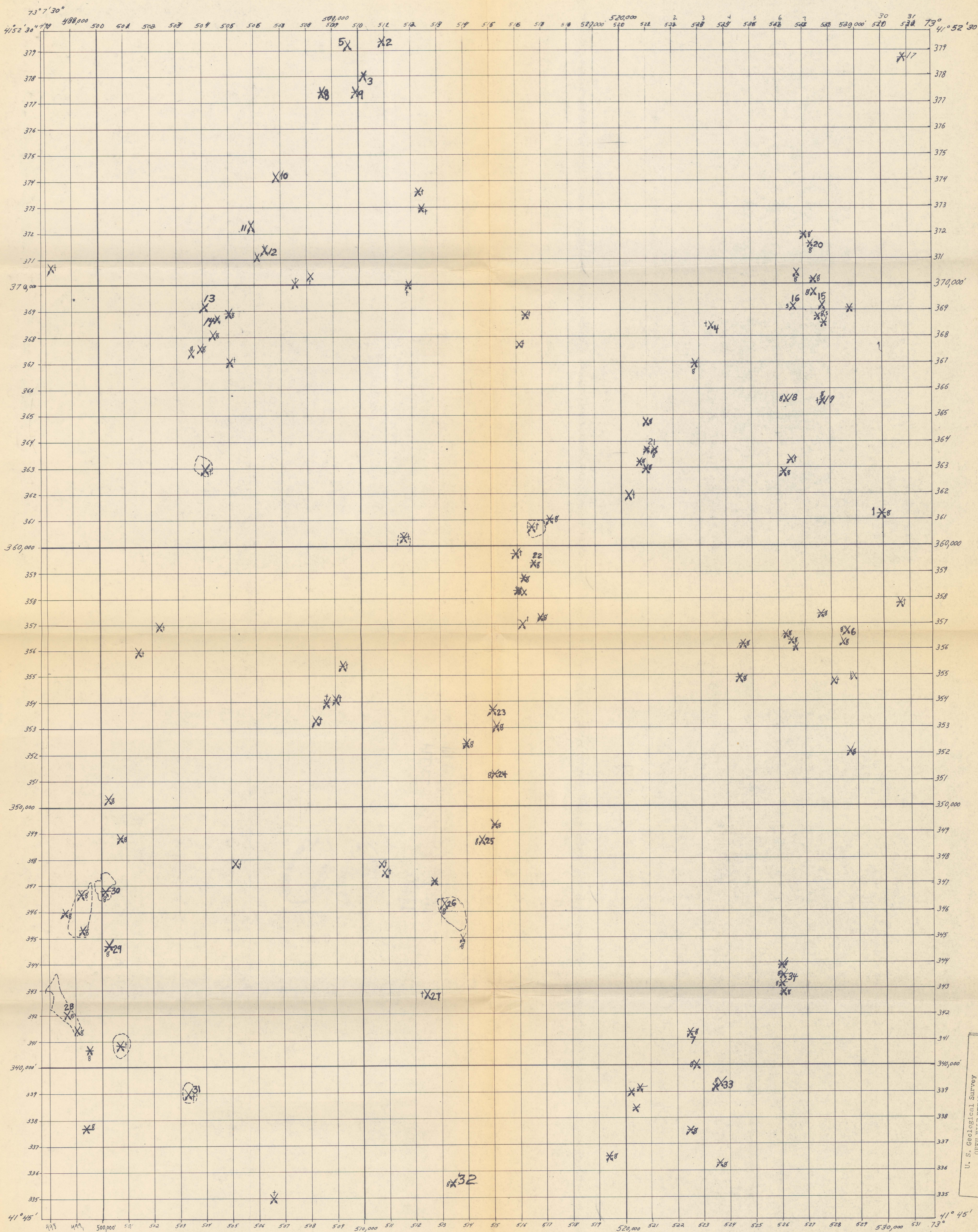
MAP SHOWING LOCATION OF SAND, GRAVEL, AND BORROW PITS TORRINGTON QUADRANGLE, CONNECTICUT BY ROGER B. COLTON 1967
