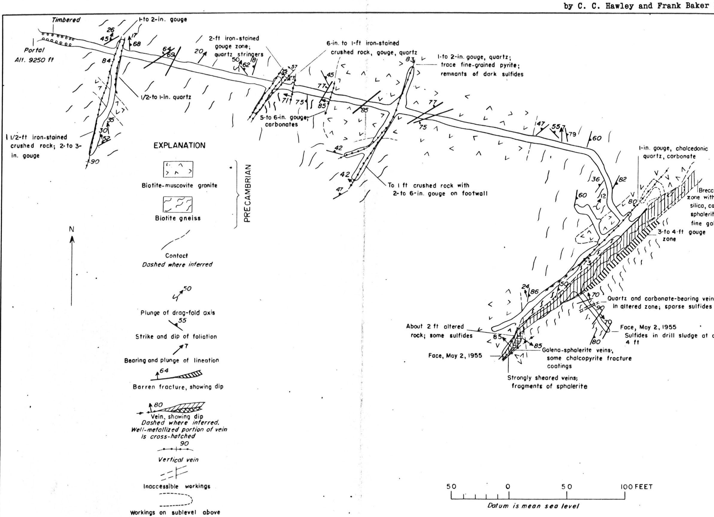
FIGURE 29.—GEOLOGIC MAP OF THE WATT STEMBLE MINE
