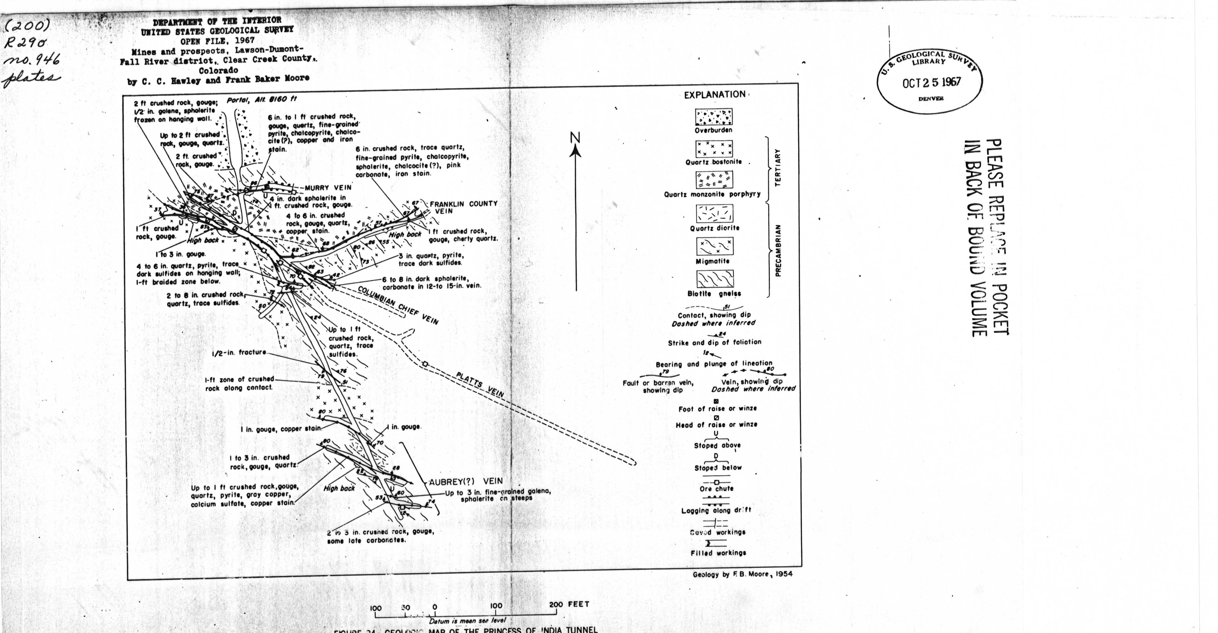
FIGURE 24.—GEOLOGIC MAP OF THE PRINCESS OF INDIA TUNNEL
