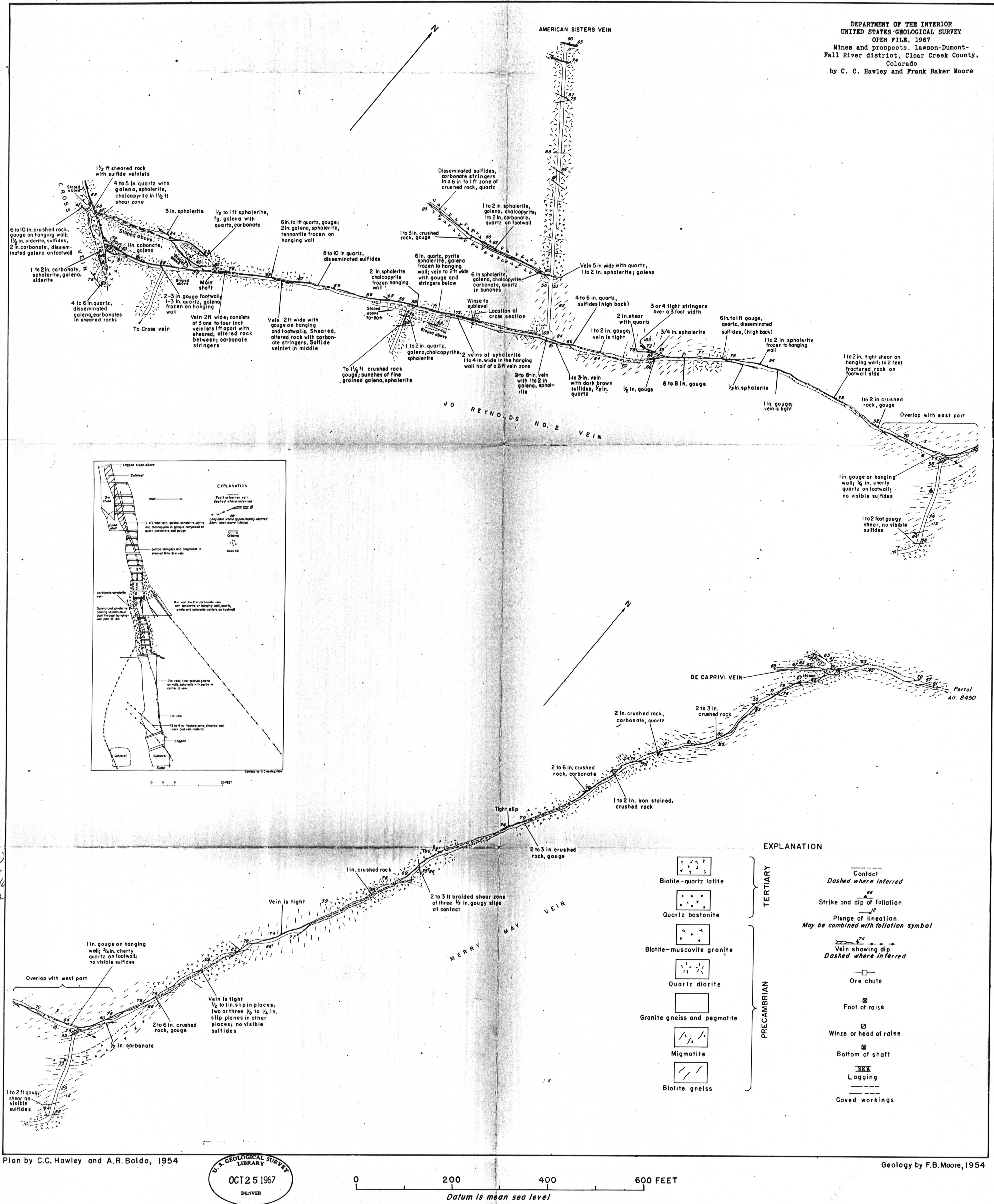
FIGURE 22.—GEOLOGIC MAP AND SECTION OF THE ELIDA TUNNEL LEVEL, JO REYNOLDS MINE
