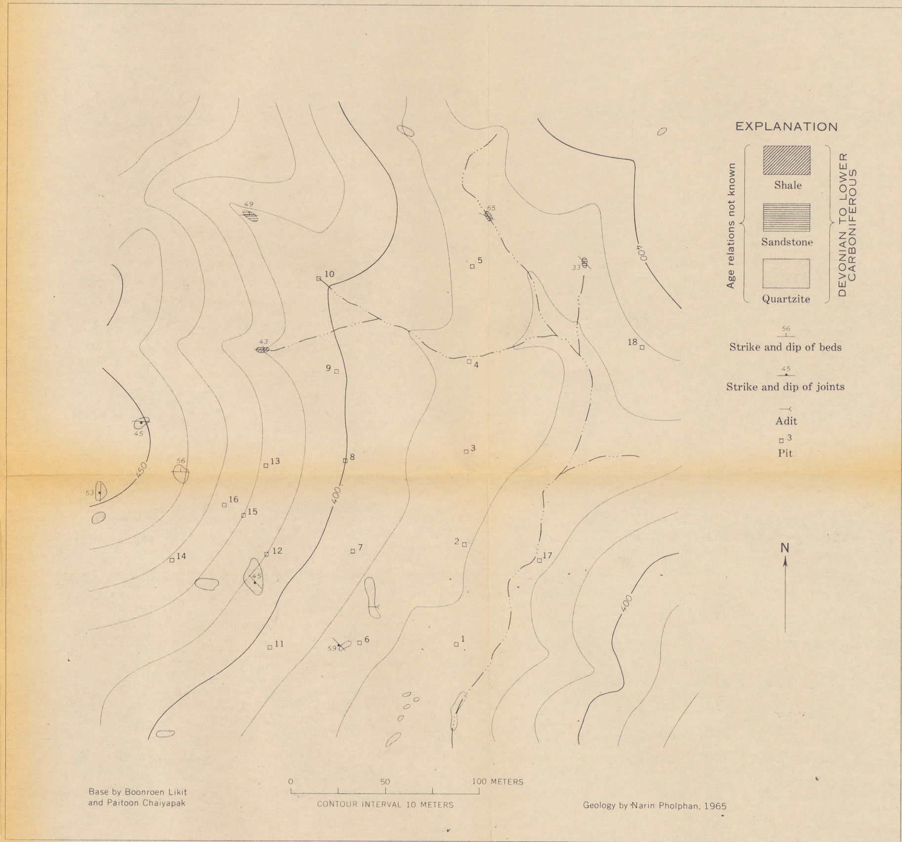
B. GEOLOGIC SKETCH MAP OF THE HUAI MUANG MANGANESE AREA
