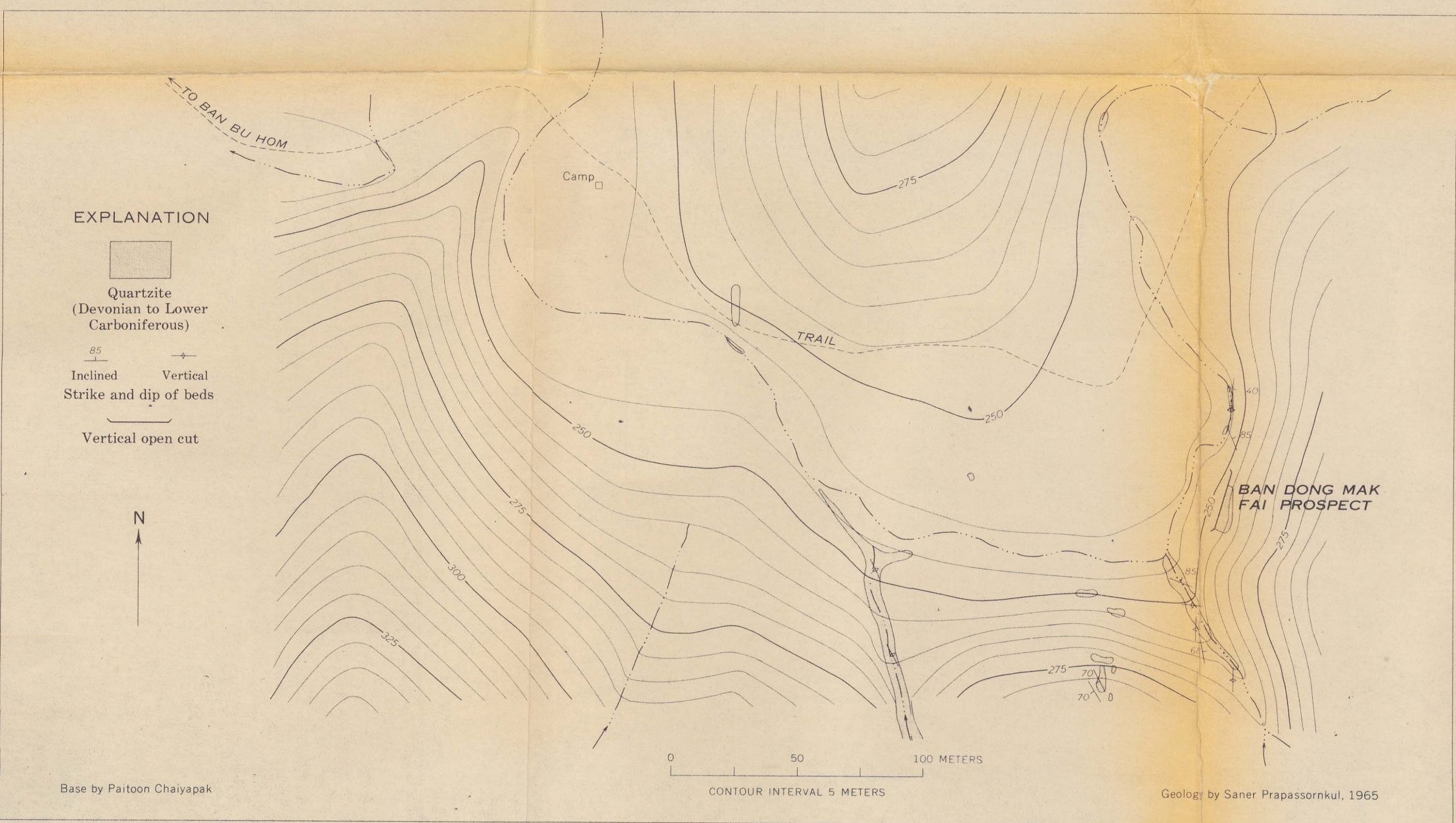
E. GEOLOGIC SKETCH MAP OF THE BAN DONG MAK FAI AREA SHOWING LOCATION OF MANGANESE PROSPECT
