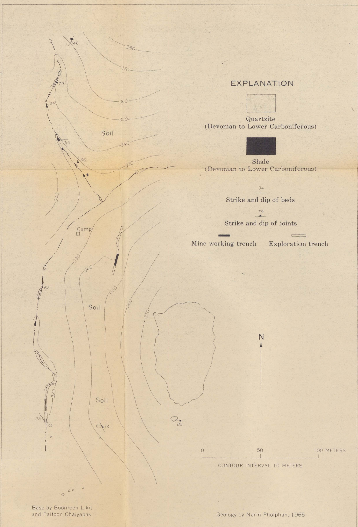
C. GEOLOGIC SKETCH MAP OF THE HUAI KHOK KHA MINE
