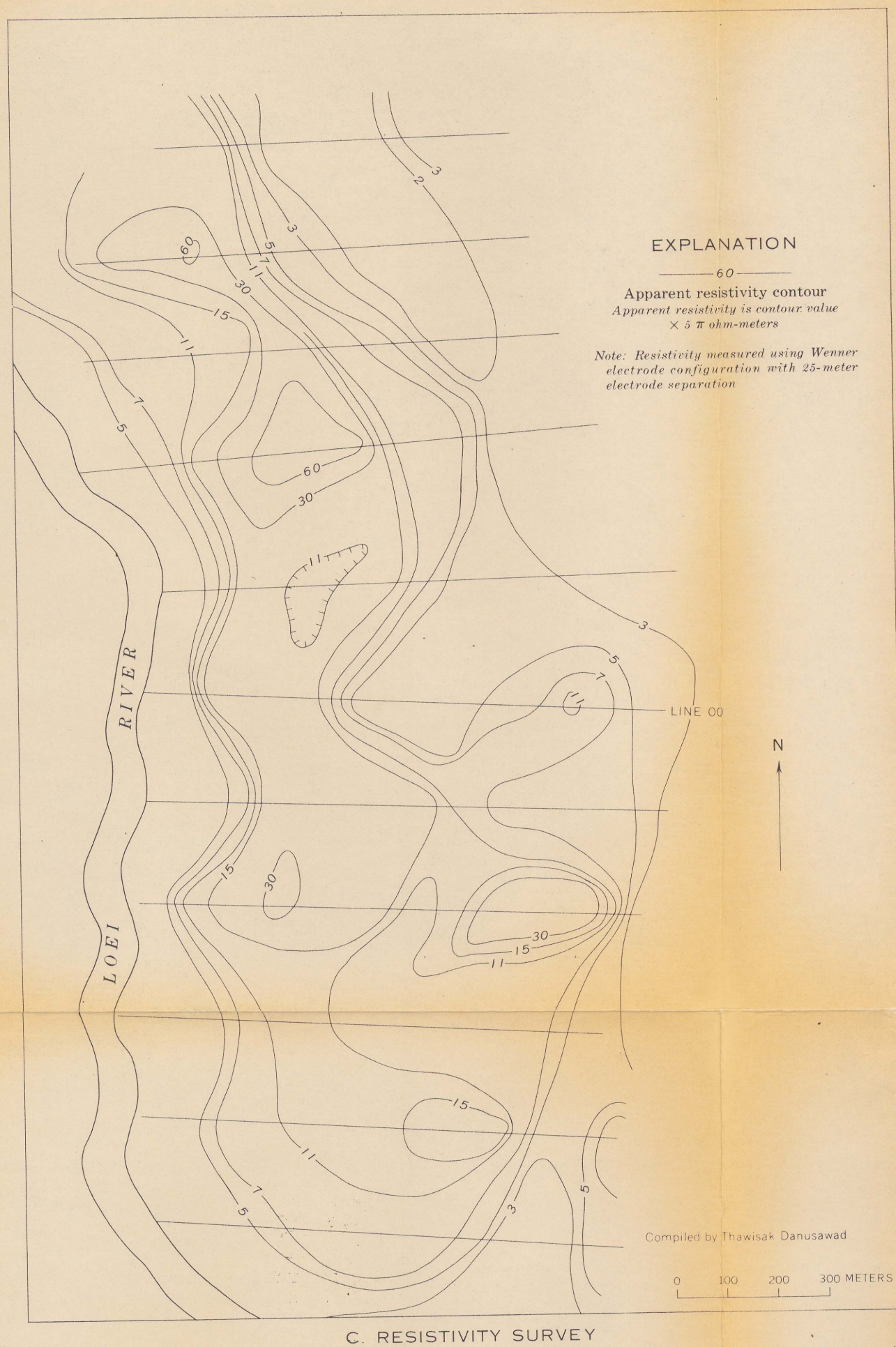
PLATE 4. MAPS AND SECTION OF THE PHU THONG DAENG BASE-METAL PROSPECT
