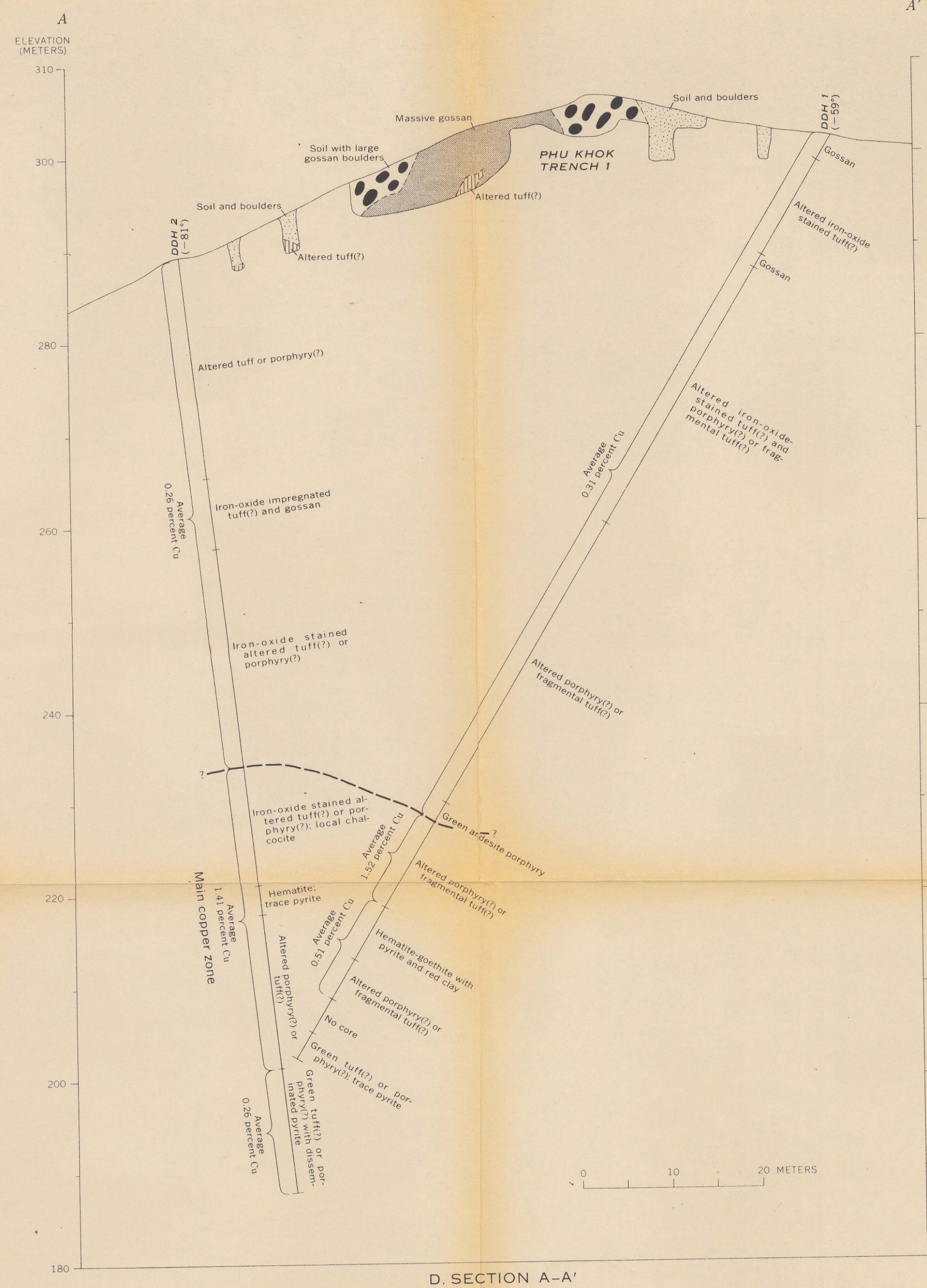
PLATE 4. MAPS AND SECTION OF THE PHU THONG DAENG BASE-METAL PROSPECT
