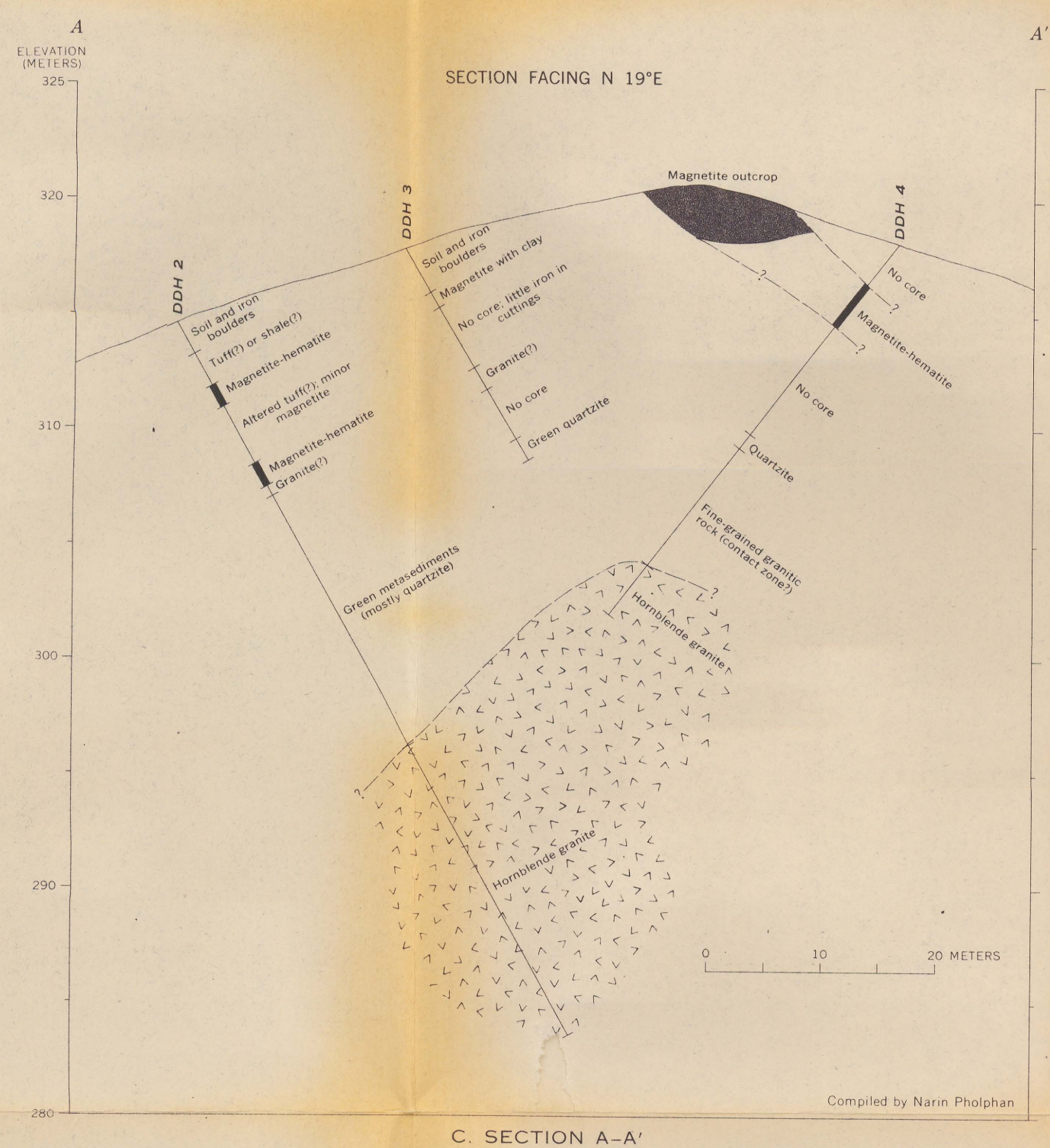
C. SECTION A-A'
