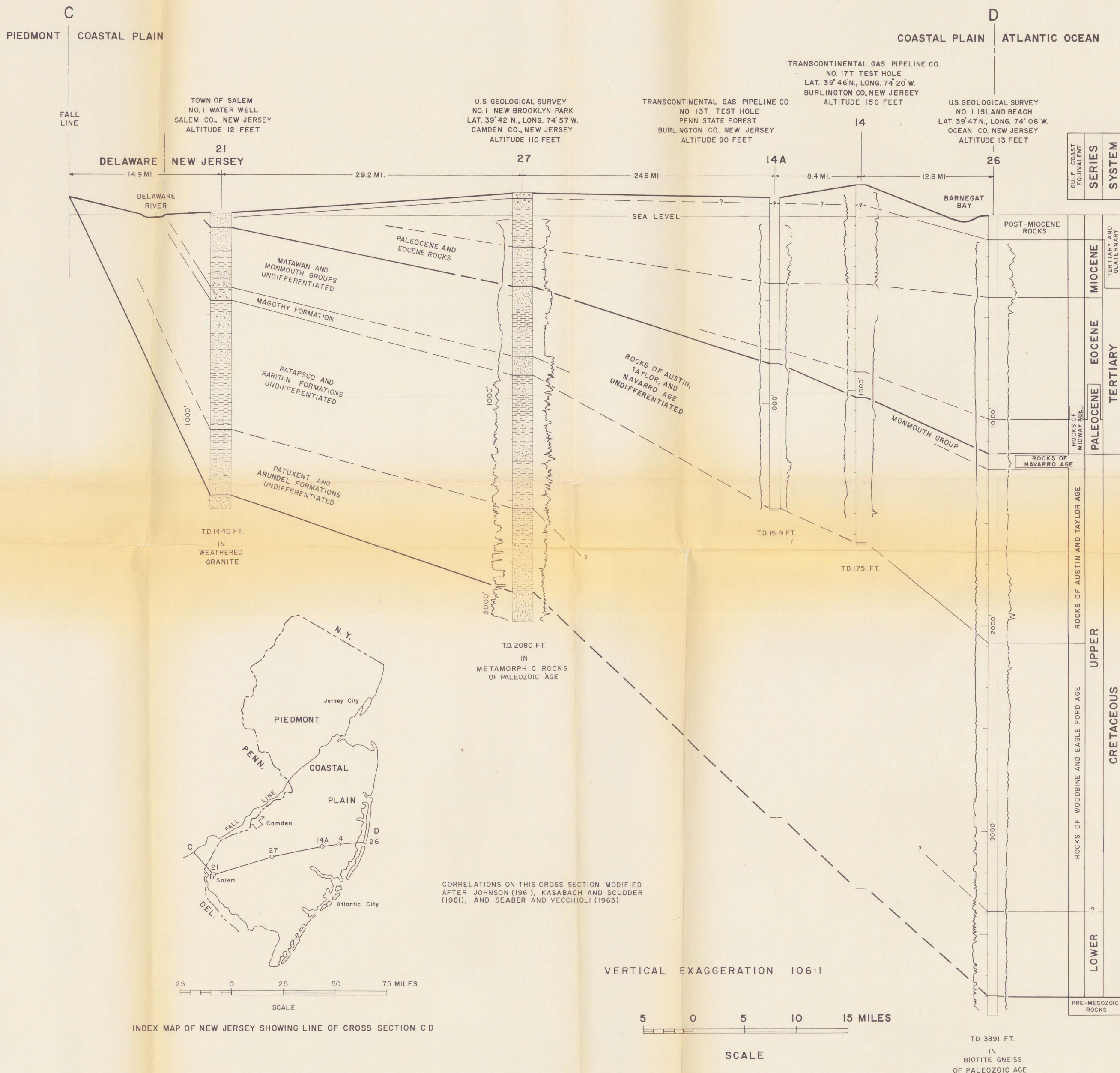
PL.10 GEOLOGIC CROSS SECTION CD OF MESOZOIC AND CENOZOIC ROCKS FROM THE FALL LINE TO THE ATLANTIC OCEAN IN NEW JERSEY
