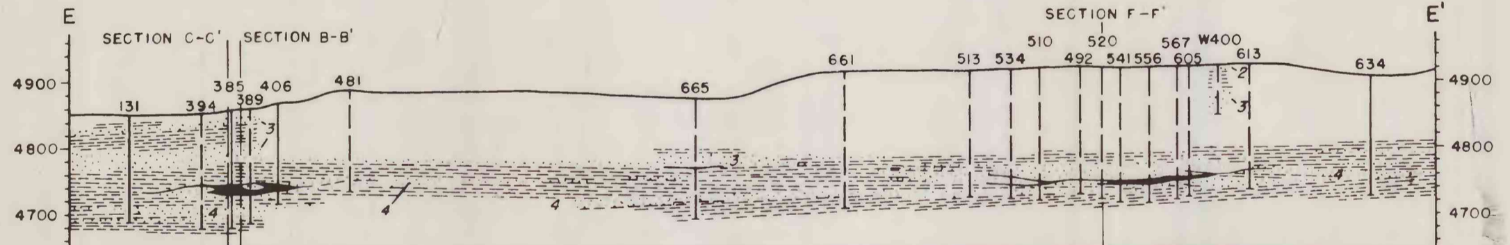
GEOLOGIC SECTION E-E'
