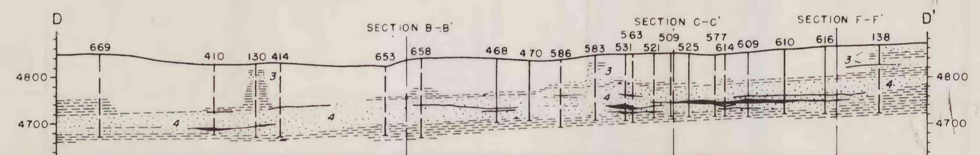
GEOLOGIC SECTION D-D'
