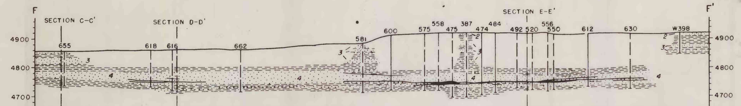
GEOLOGIC SECTION F-F'
