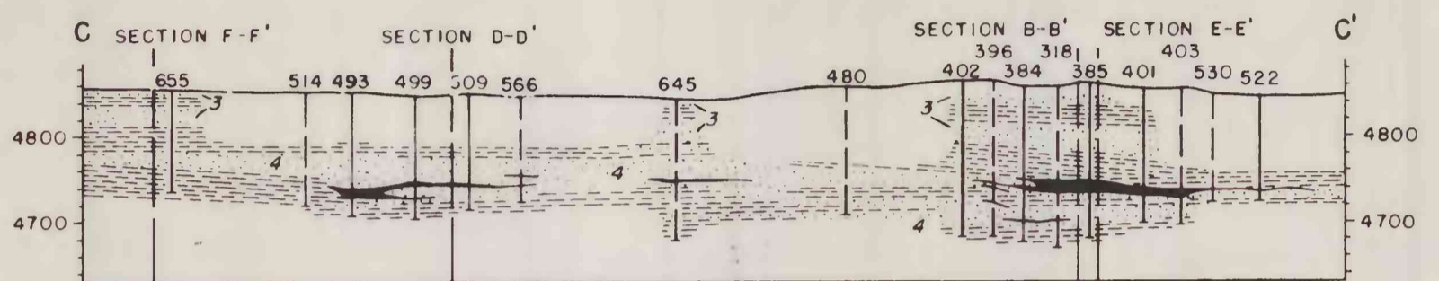
GEOLOGIC SECTION C-C'
