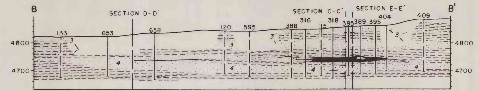
GEOLOGIC SECTION B-B'
