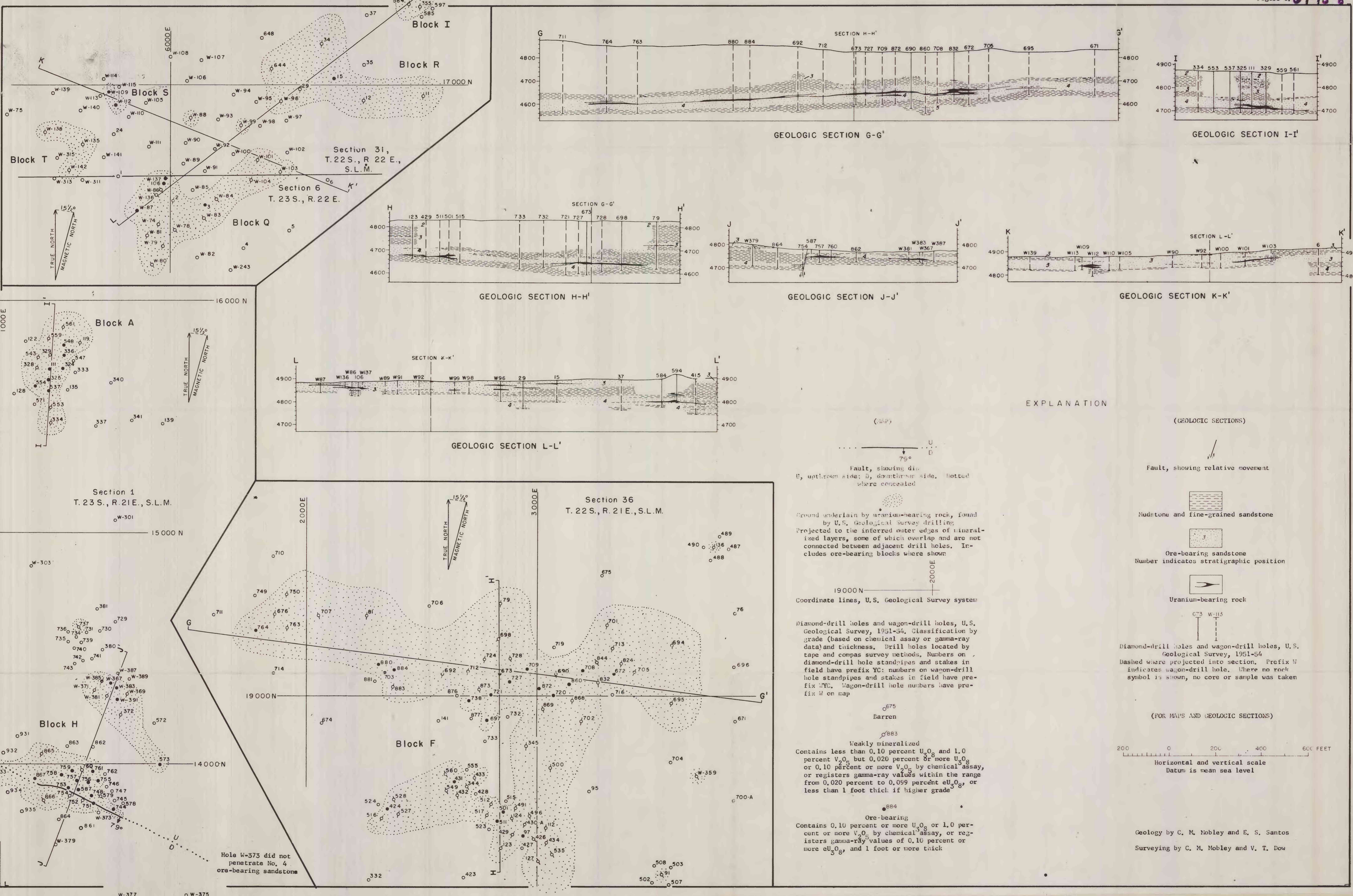
Figure 8.--MAP AND GEOLOGIC SECTIONS OF ORE-BEARING BLOCKS A, F, H, I, Q, R, S, AND T, YELLOW CAT AREA, THOMPSON DISTRICT, GRAND COUNTY, UTAH.
