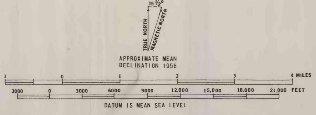
MAP OF PART OF EDWARDS AIR FORCE BASE AND VICINITY, CALIFORNIA SHOWING WATER-LEVEL CHANGE MARCH 1961 TO MARCH 1967
