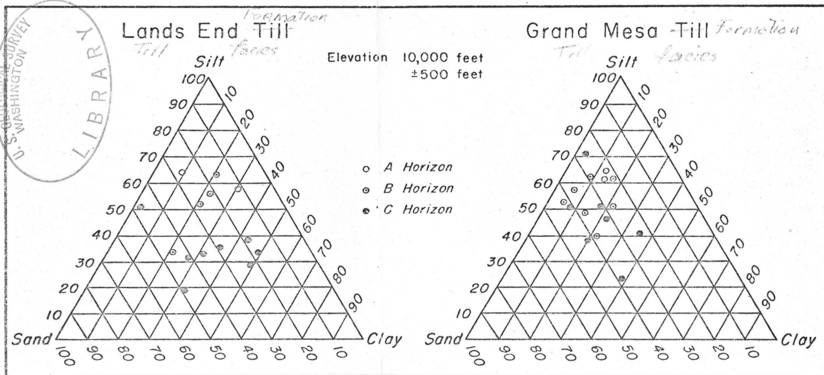
Figure 11.--Texture triangle diagrams showing percentages of sand, silt, and clay in the matrix of the tills of the Lands End and Grand Mesa Formations. Percentages are also shown for some of the respective soil horizons developed on the tills. Mechanical analyses were determined by hydrometer. Sand, silt, and clay were calculated as a percent of the 2-mm fraction.
