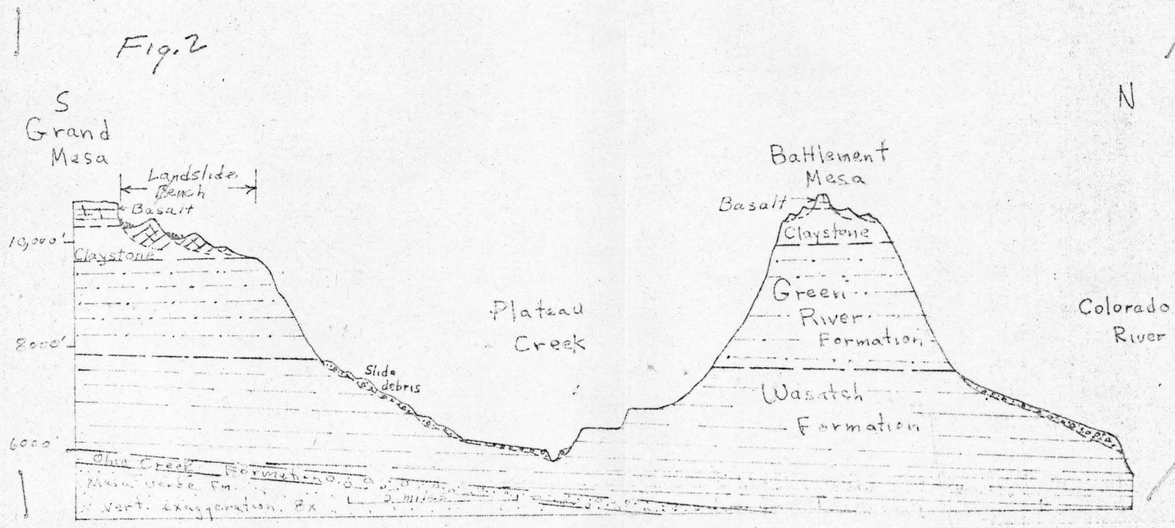
Figure 2.--Diagrammatic cross section from Grand Mesa through Battlement Mesa to the Colorado River.
