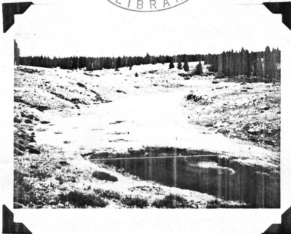
Figure 23 21.--Pre-glacial drainage of Kahnah Creek on surface of Grand Mesa.
