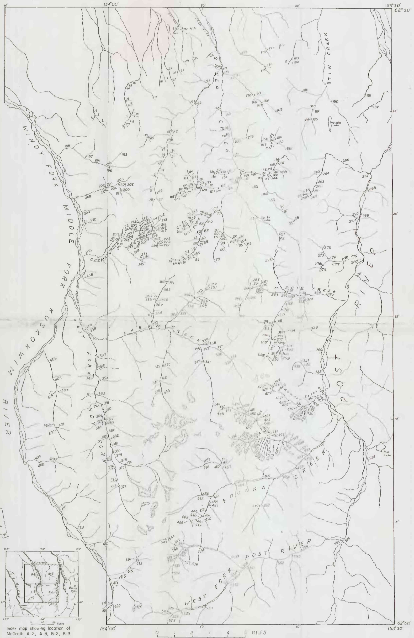
Figure 1. Location of stream-sediment samples between Windy Fork and Post River, Southern Alaska Range
