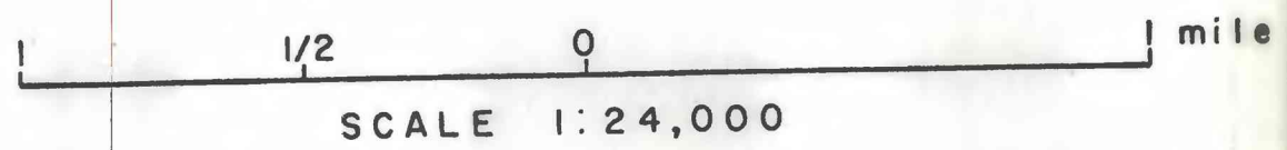
Fig. 2c. Geochemical Map Showing Concentration of Lead in the "Thrust Belt"
