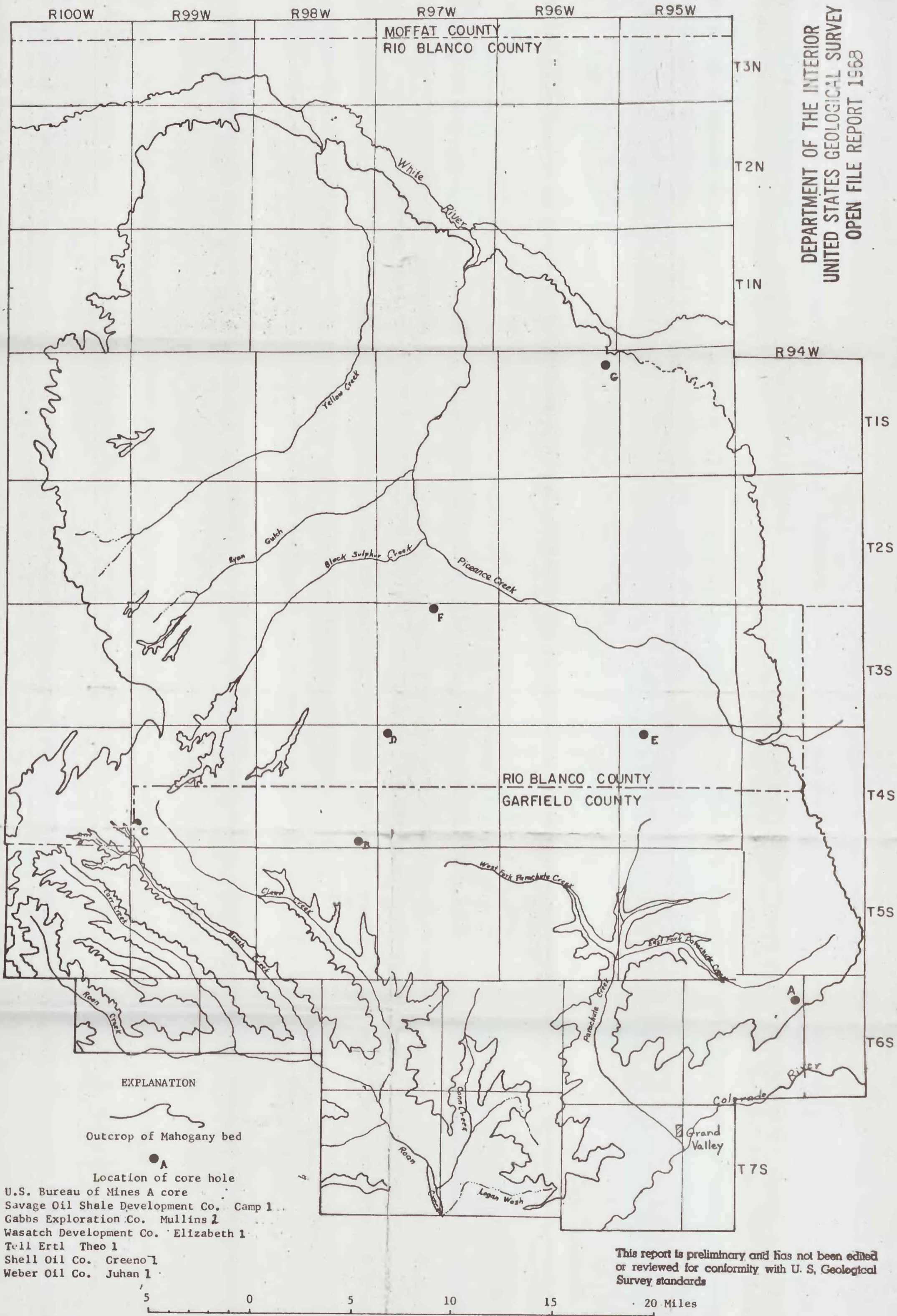
Plate 1.--Outline of the part of the Piceance Creek Basin between the Colorado and White Rivers showing the location of cores studied .
