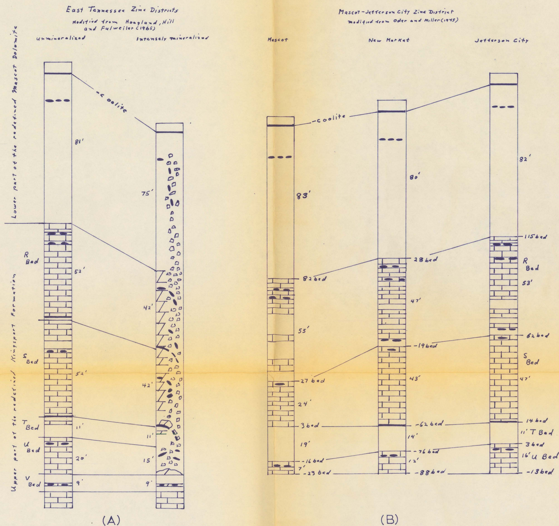
Figure 6. Diagram showing solution-thinning and collapse features in the upper part of the Kingsport Formation and the lower part of the Mascot Dolomite. (A) Relationships in a collapse zone and (B) solution-thinning of limestone in the Mascot-Jefferson City zinc district.
