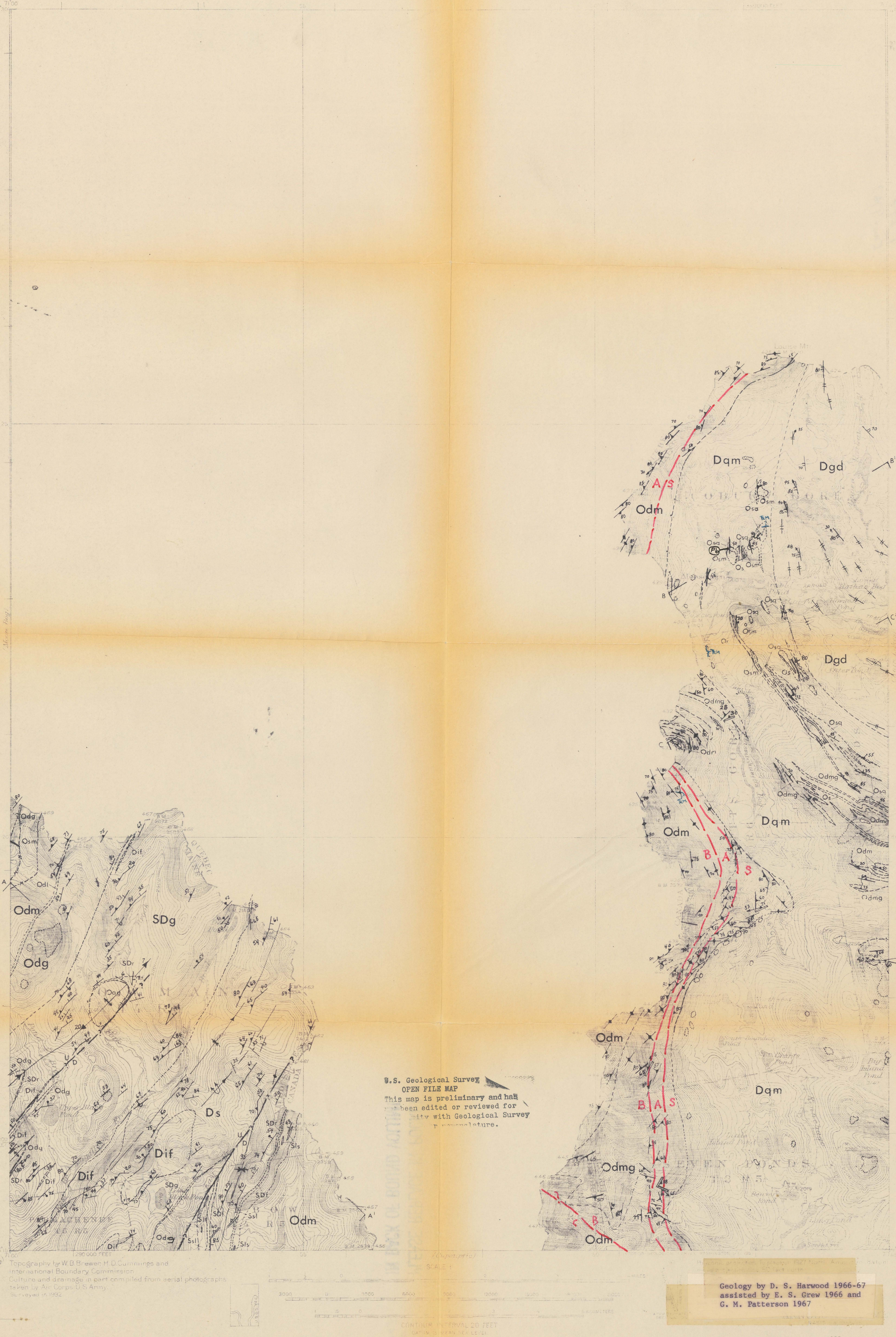
GEOLOGIC MAP OF THE ARNOLD POND QUADRANGLE, MAINE
