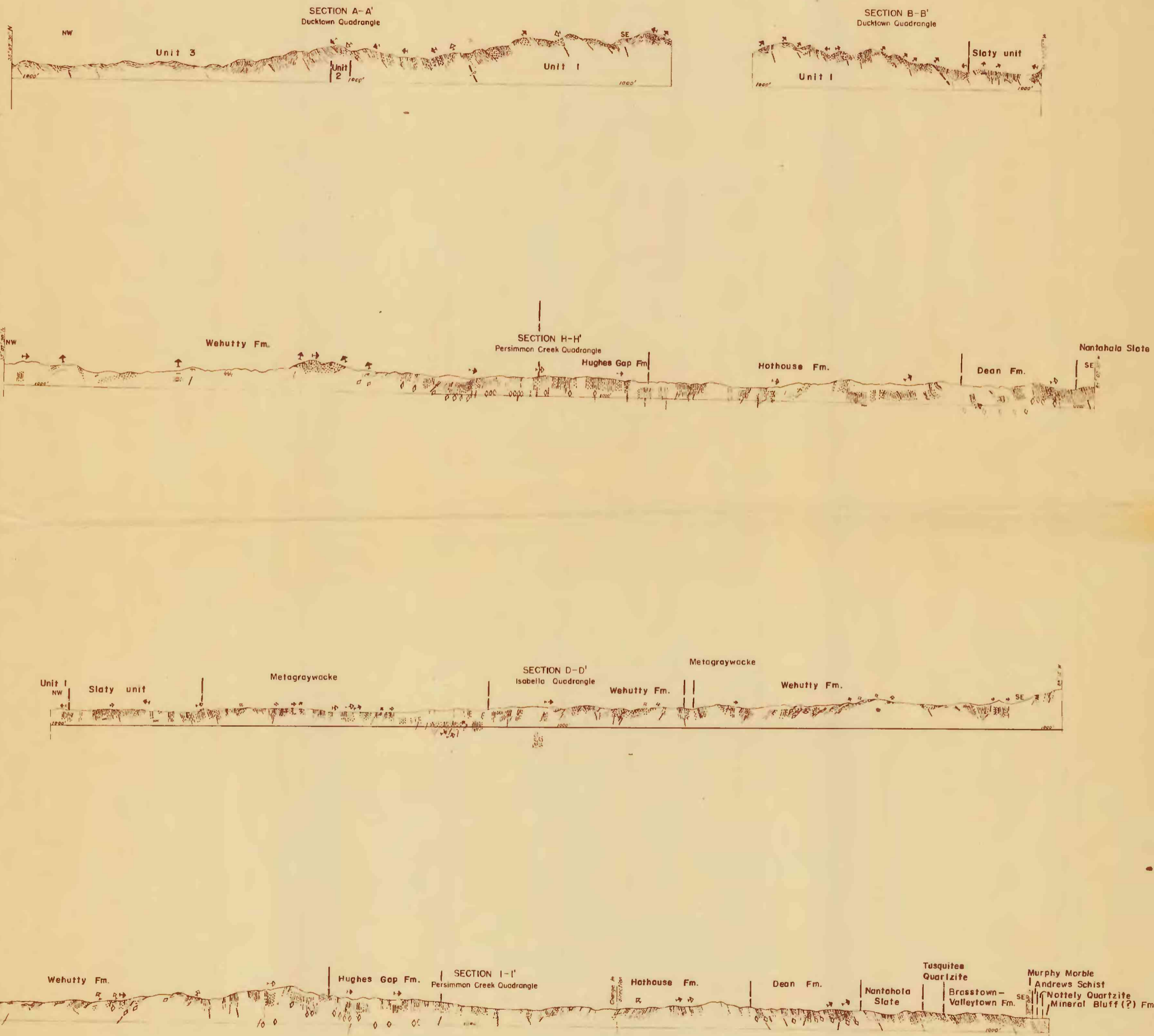
GEOLOGIC SECTIONS TO ACCOMPANY FIGURE 1, GEOLOGIC MAP OF THE DUCKTOWN, ISABELLA, AND PERSIMMON CREEK QUADRANGLES, TENNESSEE AND NORTH CAROLINA
