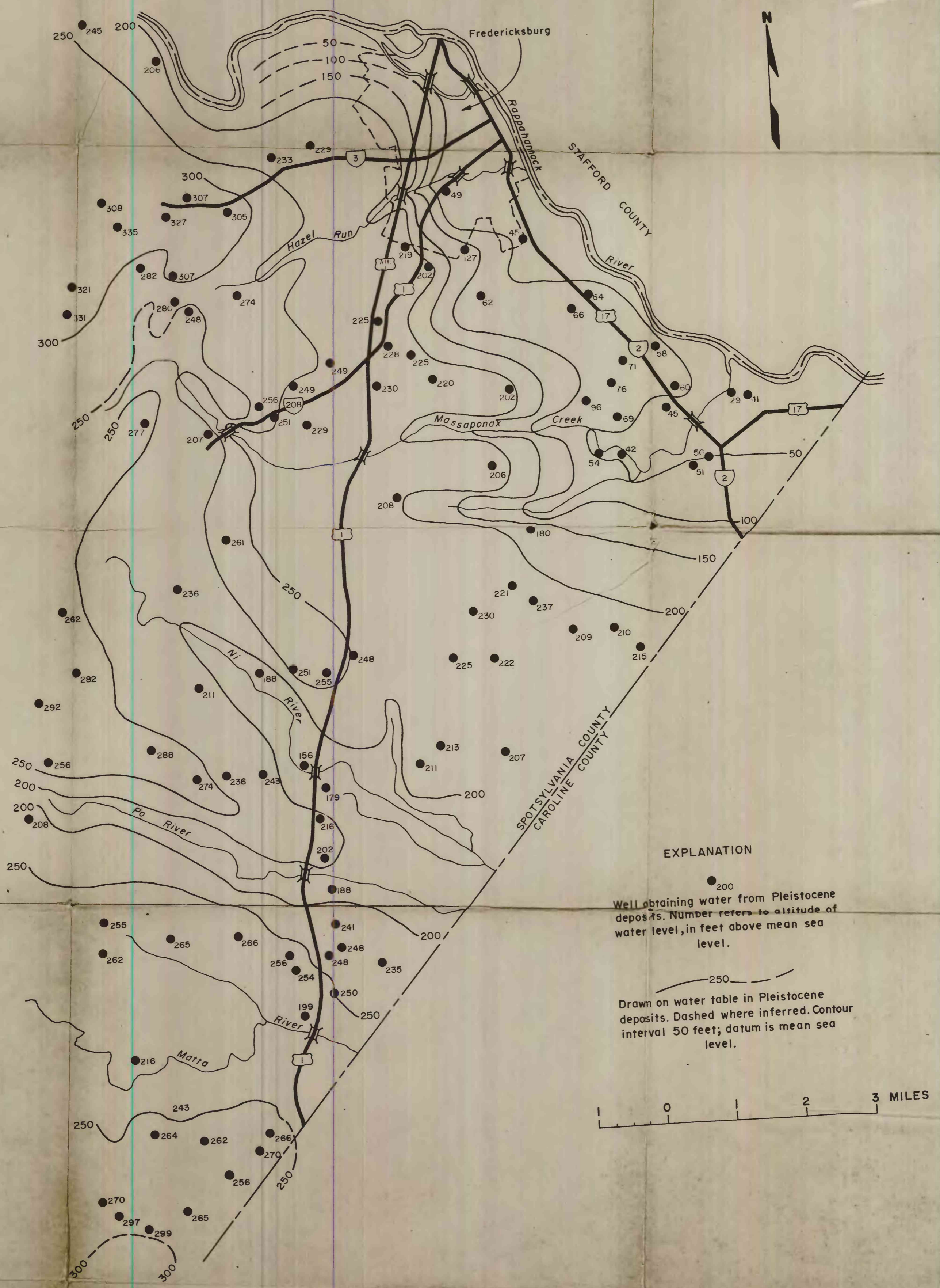
Figure 7.--Map of Coastal Plain province, Spotsylvania County, showing contours on the water table, October 1955.
