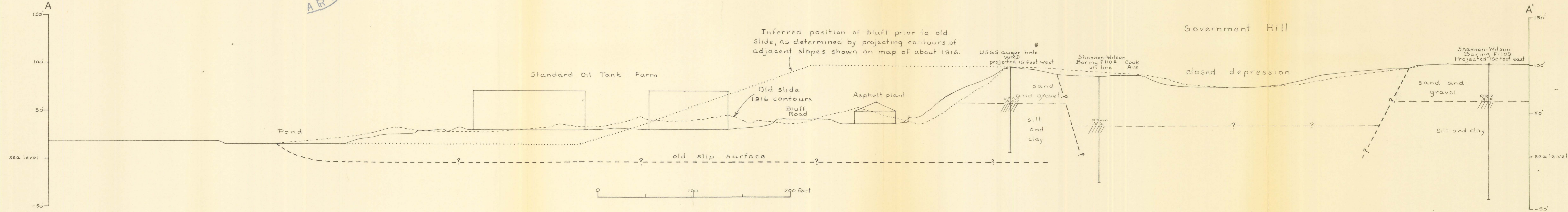
Figure 20 Section A-A' through old slide and the closed depression on Government Hill
