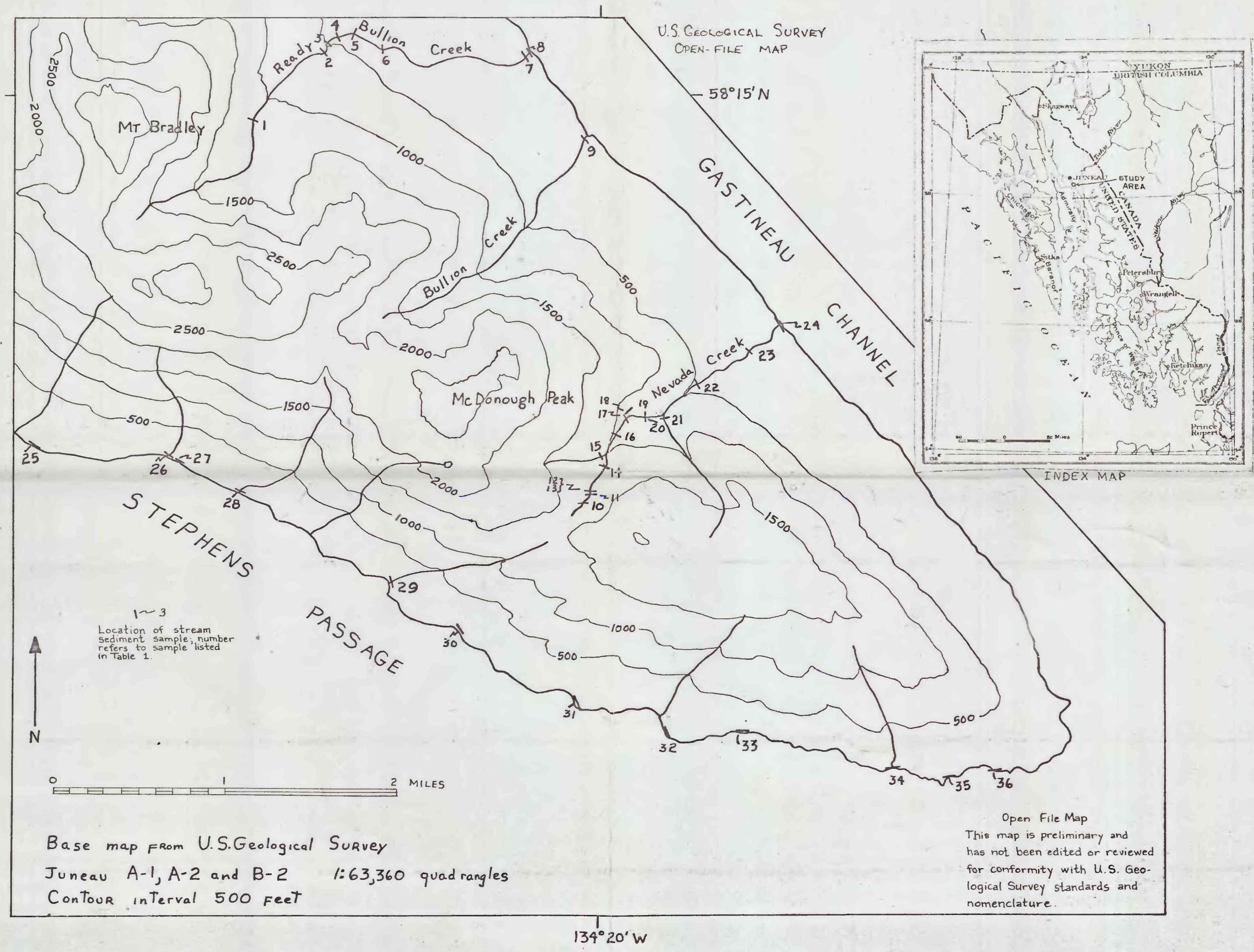
Figure 1-- Location of stream-sediment samples on southeastern Douglas Island, southeastern Alaska.
