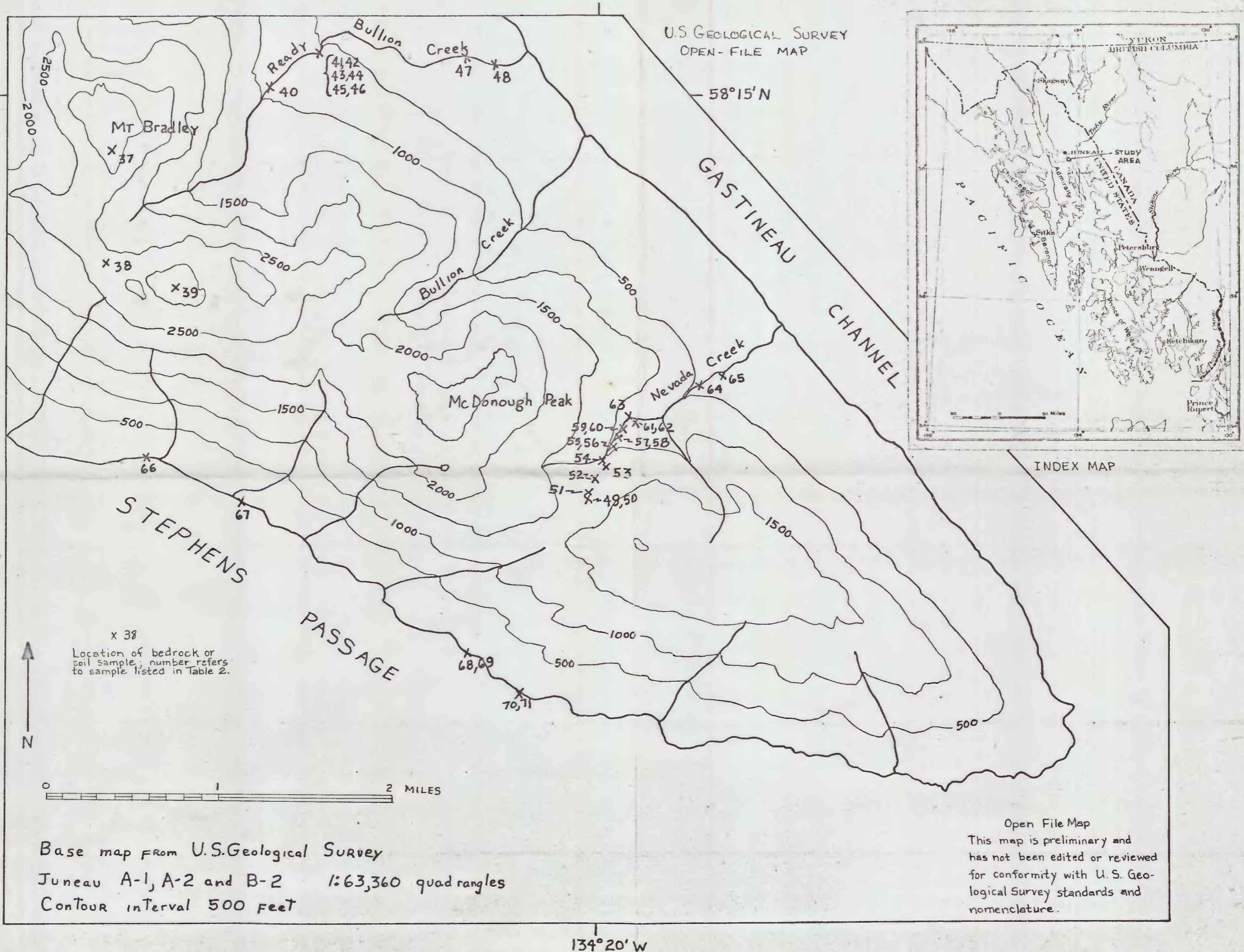
Figure 2. Location of bedrock and soil samples on southeastern Douglas Island, southeastern Alaska.
