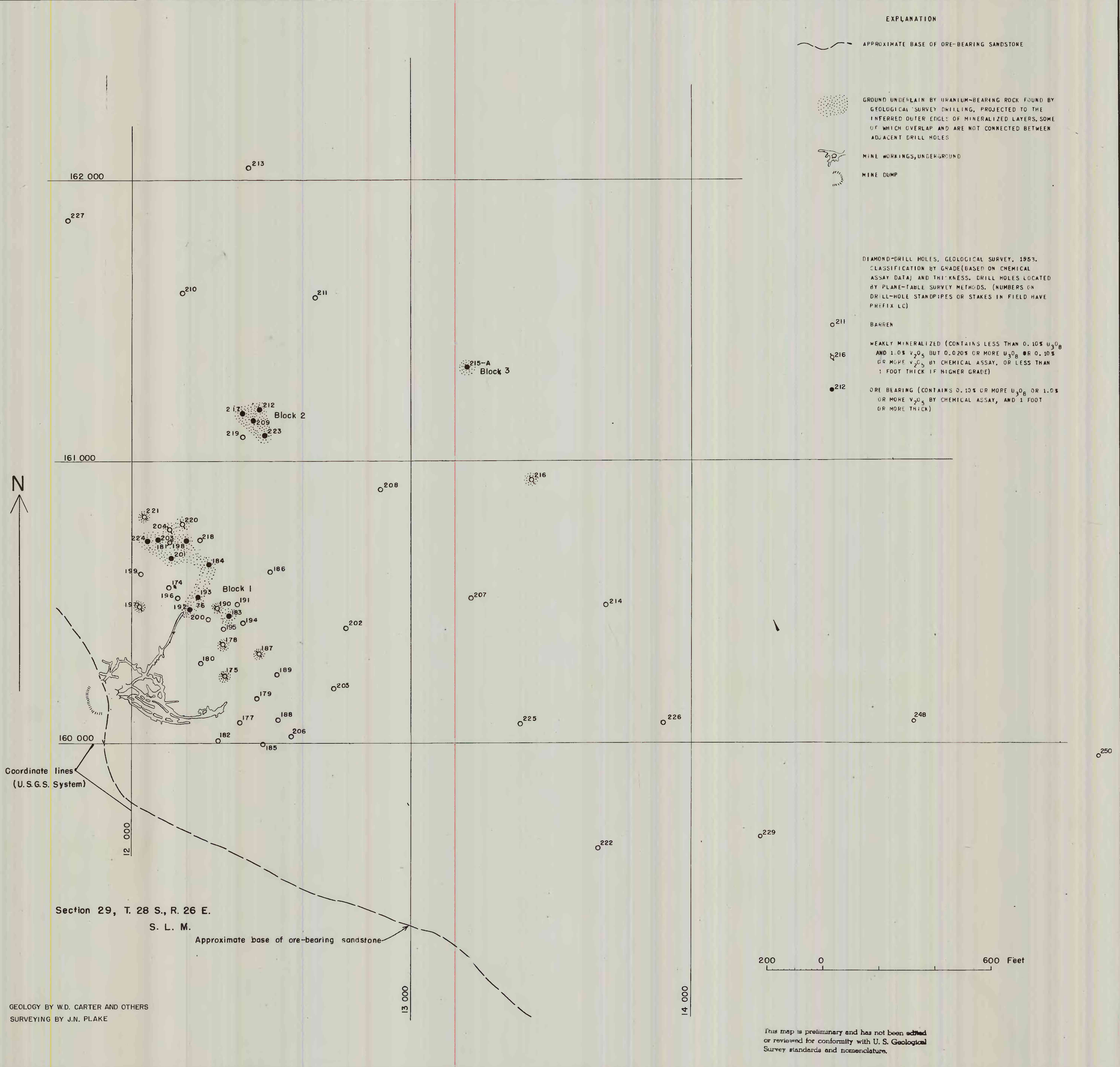
FIGURE 4.--MAP OF THE VANADIUM QUEEN GROUP VICINITY, LA SAL CREEK AREA, PARADOX DISTRICT, SAN JUAN COUNTY, UTAH
